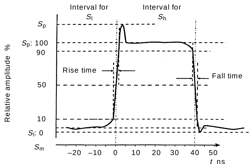
Figure 3 – Output waveform measurement
