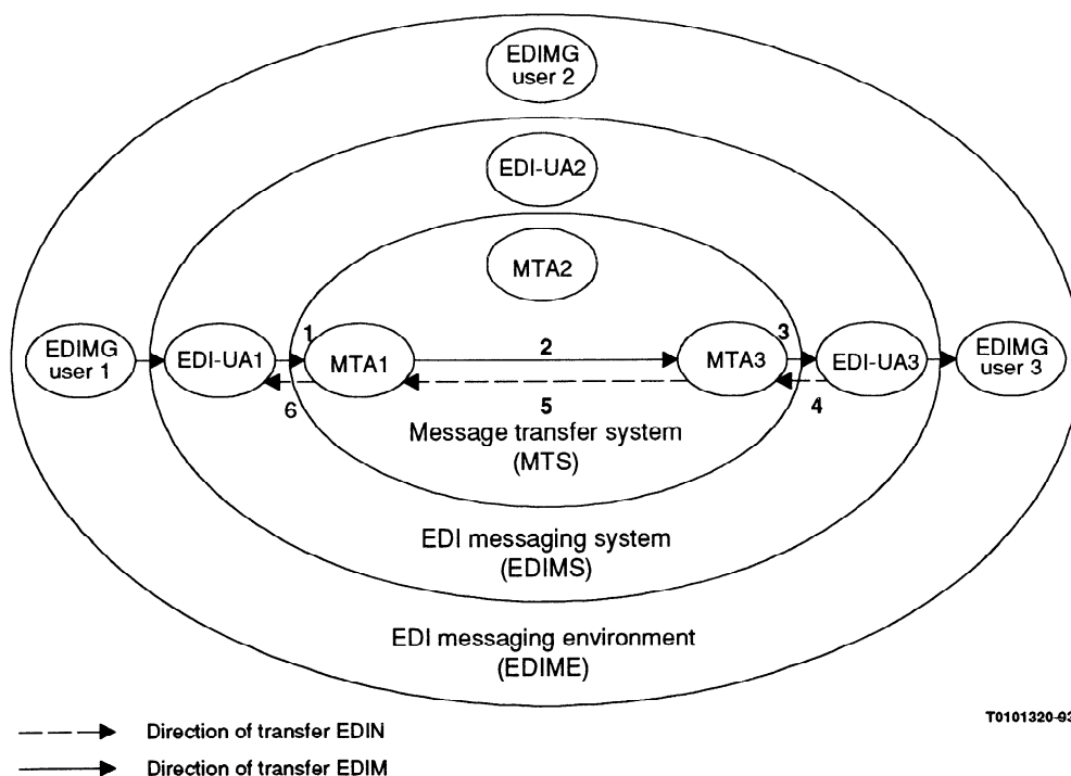
Figure 7 – Case 1: No forwarding
