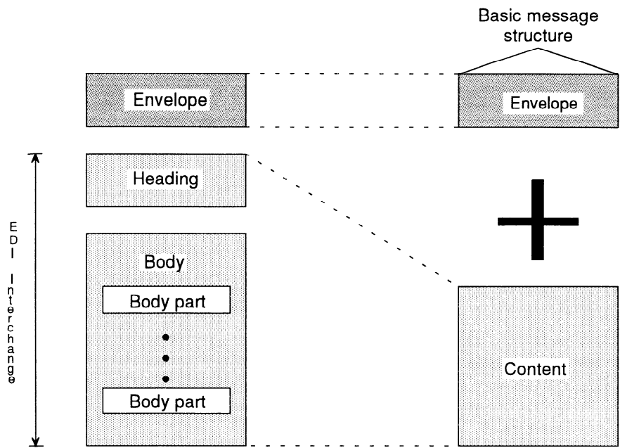
Figure 5 – EDI message structure
