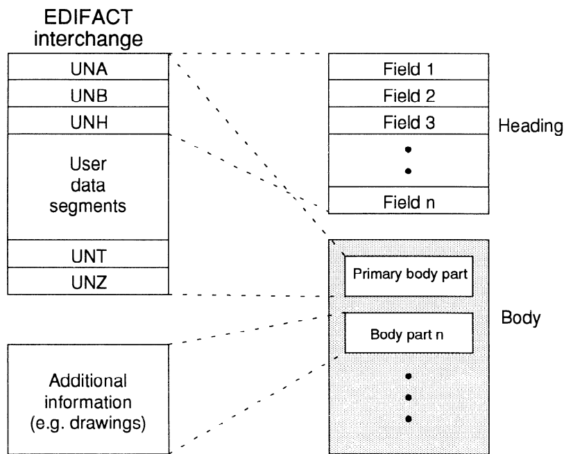
Figure 6 – EDI message structure for a typical EDI transaction
