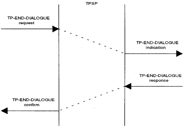
Figure 4 - Confirmed TP-END-DIALOGUE sequence of primitives
