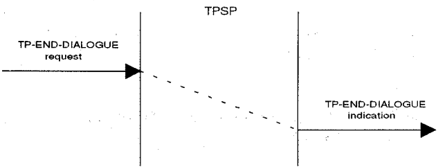
Figure 3 - Unconfirmed TP-END-DIALOGUE sequence of primitives
