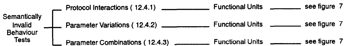
Figure 6 — Semantically Invalid Behaviour Test Group Structure (Initiator)
