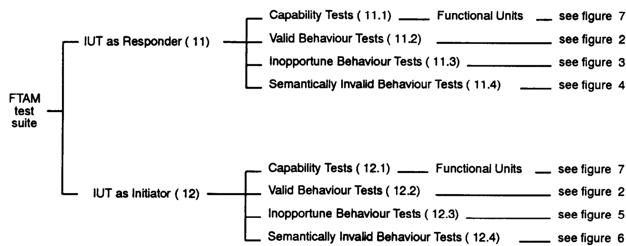
Figure 1 — FTAM Test Suite Structure
