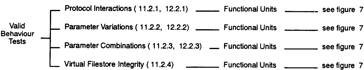
Figure 2 — Valid Behaviour Test Group Structure
