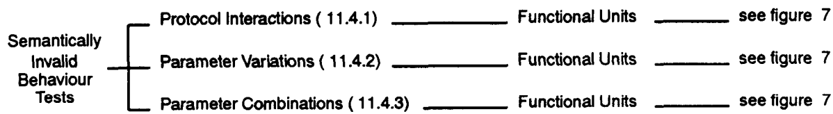
Figure 4 — Semantically Invalid Behaviour Test Group Structure (Responder)
