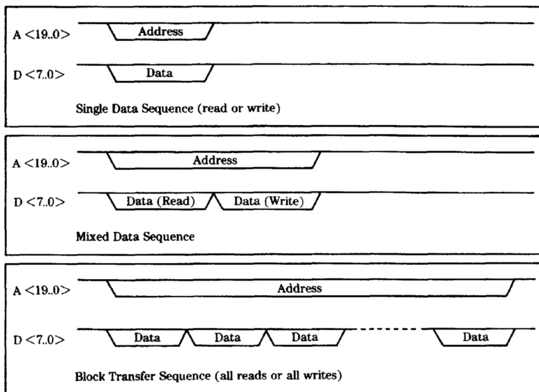
Figure 6 – IEEE Std 1000 Bus data transfer sequences
