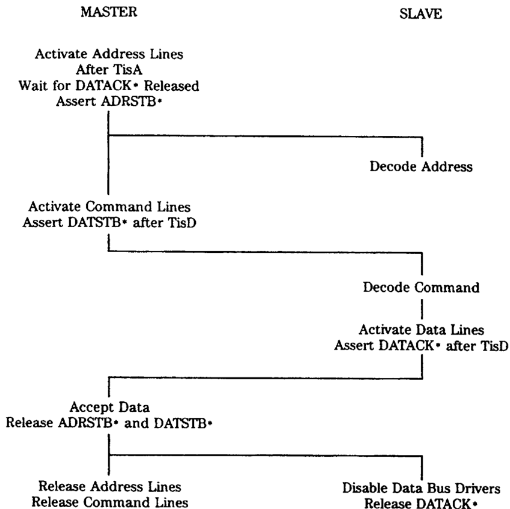
Figure 7 – Read sequence flow diagram
