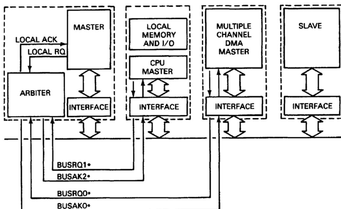
Figure 5 – Example of multiple master implementation
