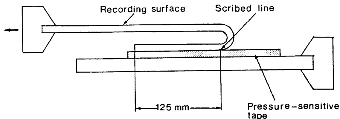
Figure 1 - Coating adhesion
