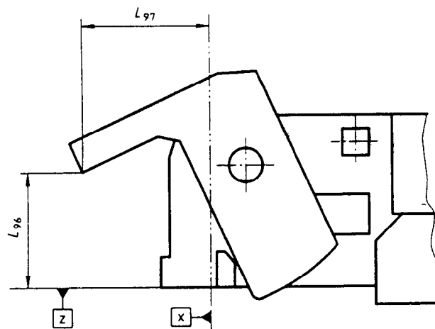
Figure 18 - Lid in completely open position
