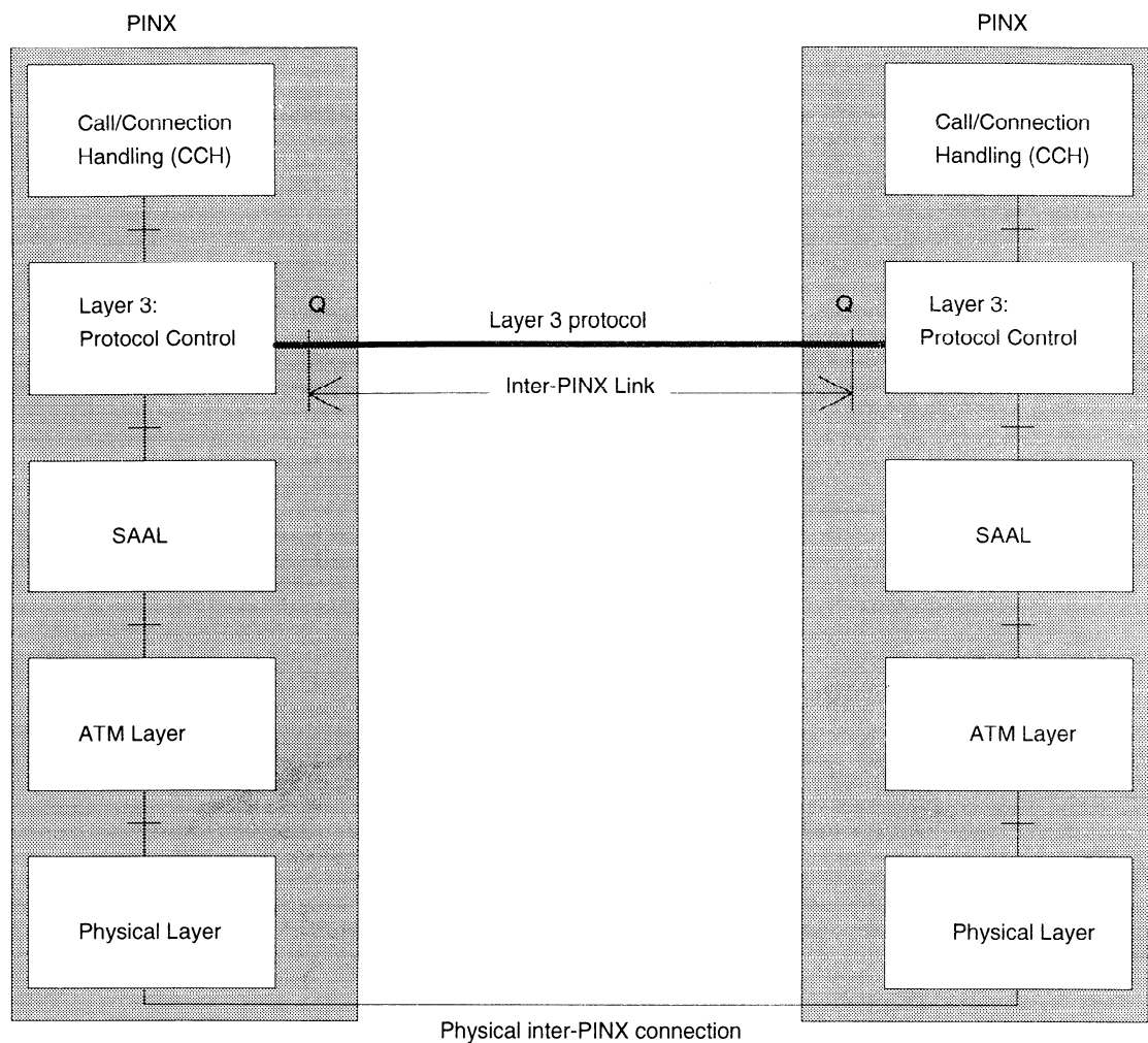
Figure 3 — Control plane protocol model
