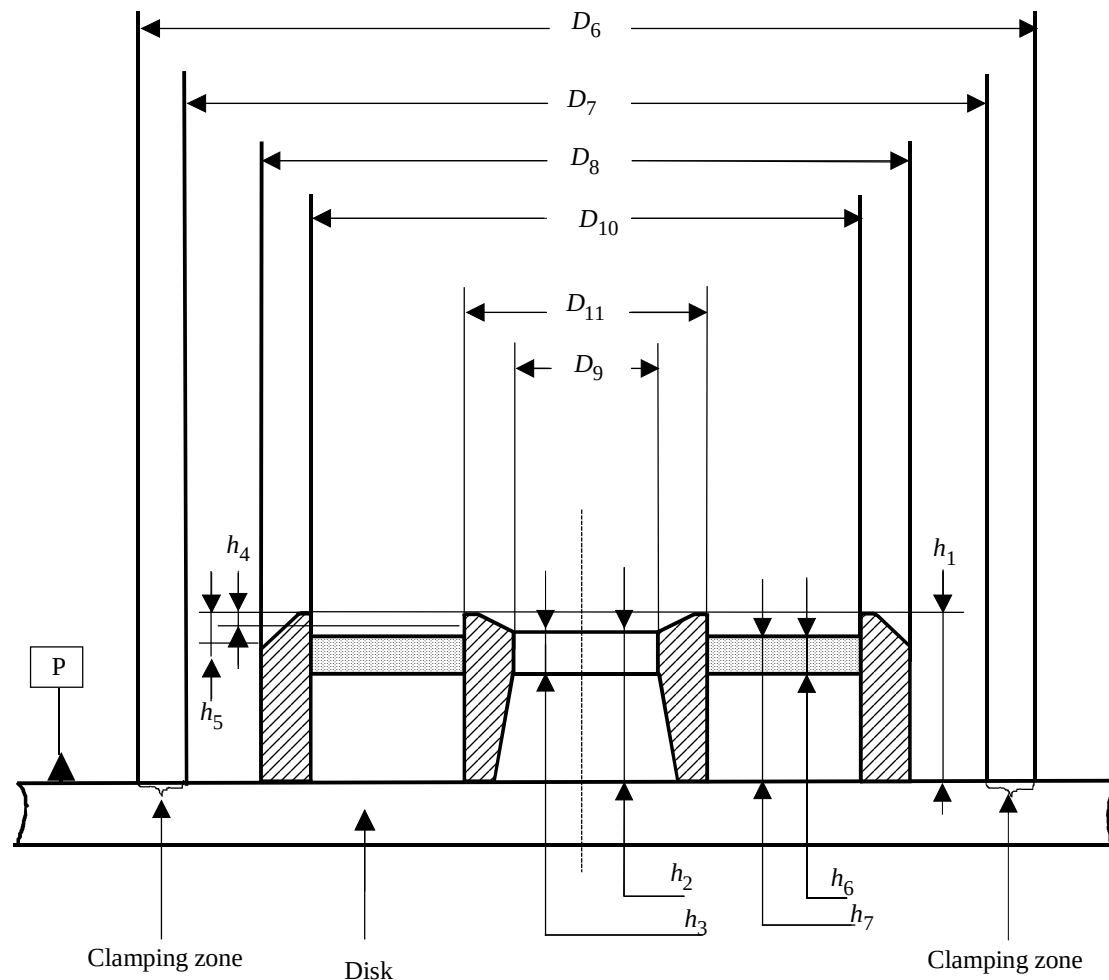
Figure 2 - Hub dimensions
