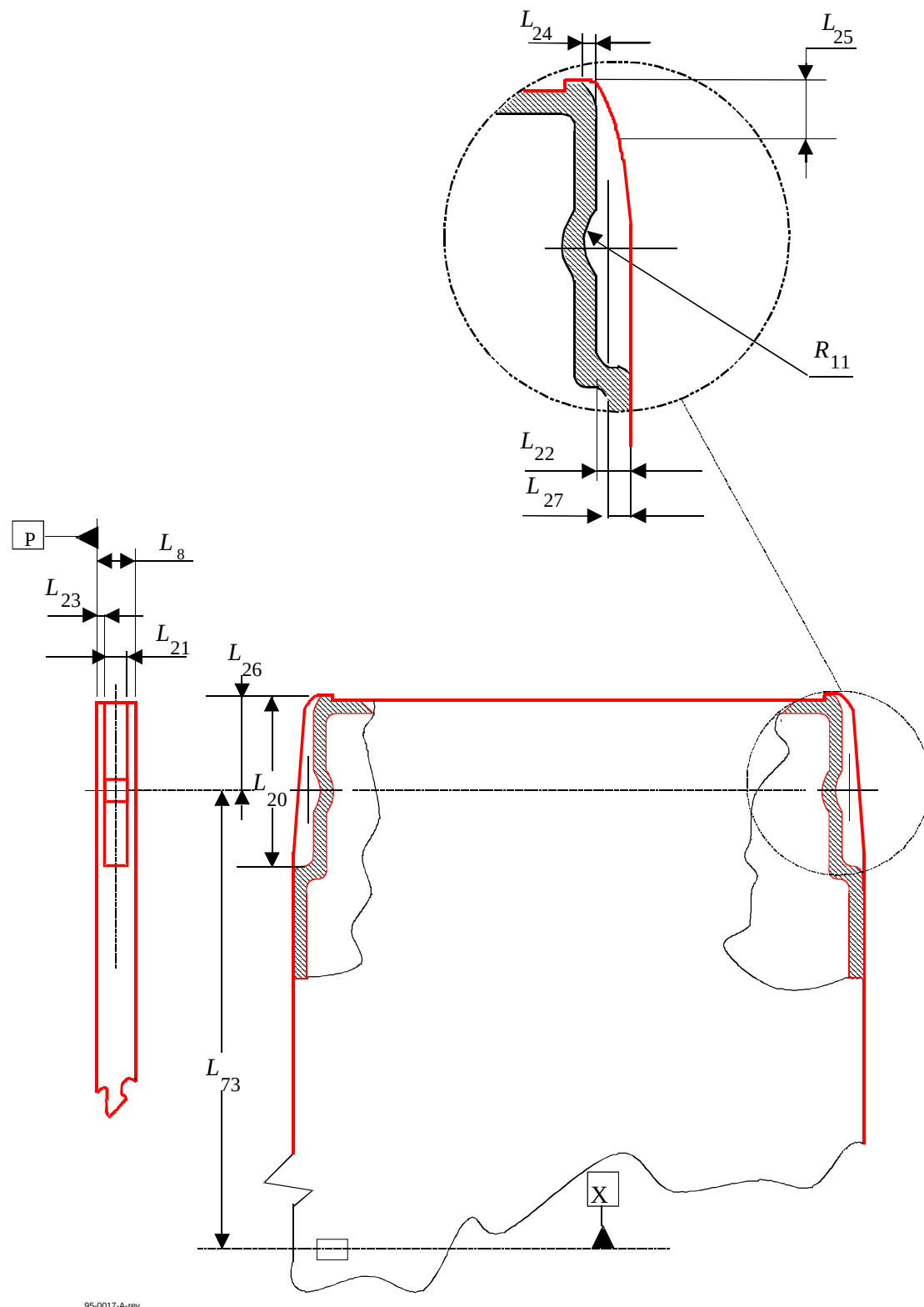
Figure 6 - Insertion slot and detent
