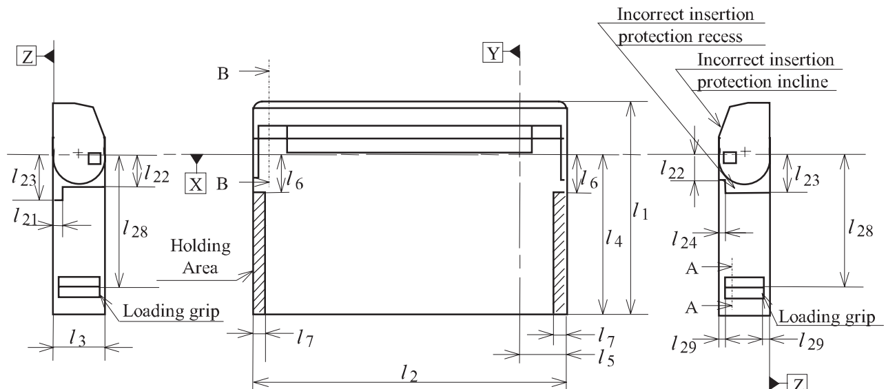
Figure 5 - Left side, lid closed
