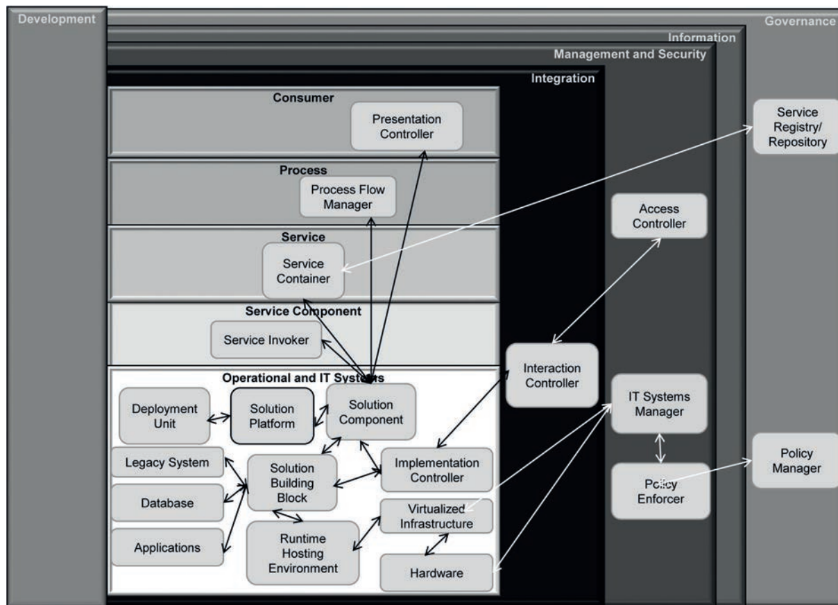
Figure 11 — Key Interactions of Operational and IT Systems Layer with Horizontal Layers
