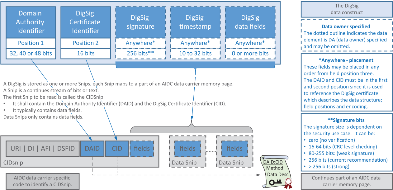
Figure 6 — The construction and mapping of an DigSig in an AIDC data carrier
