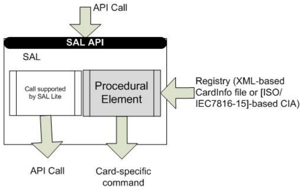
Figure D1 – Procedural Element functionality
