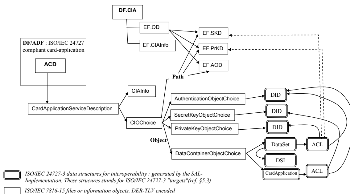
Figure 8-2 — Relationships between ISO/IEC 7816-15 information objects and ISO/IEC 24727-3 data structures
