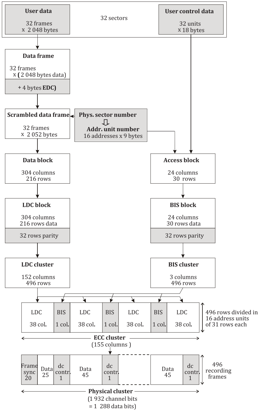
Figure 21 — Schematic representation of encoding process
