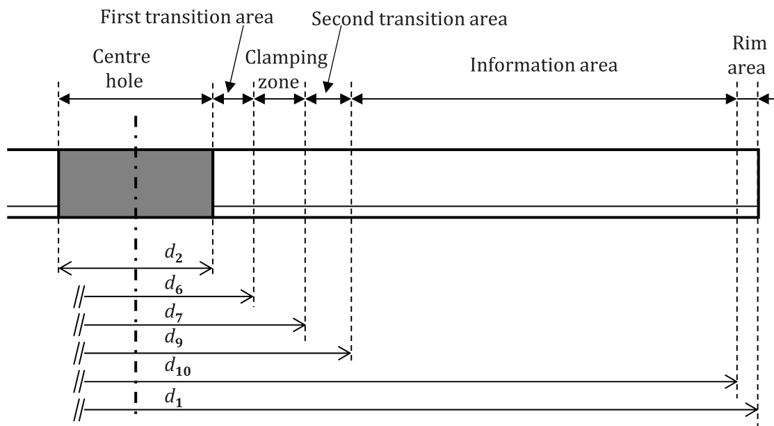
Figure 11 — Overview of disk dimensions
