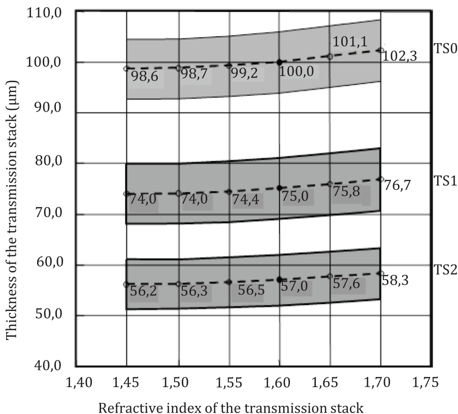
Figure 17 — Thickness of the transmission stacks as a function of the refractive index
