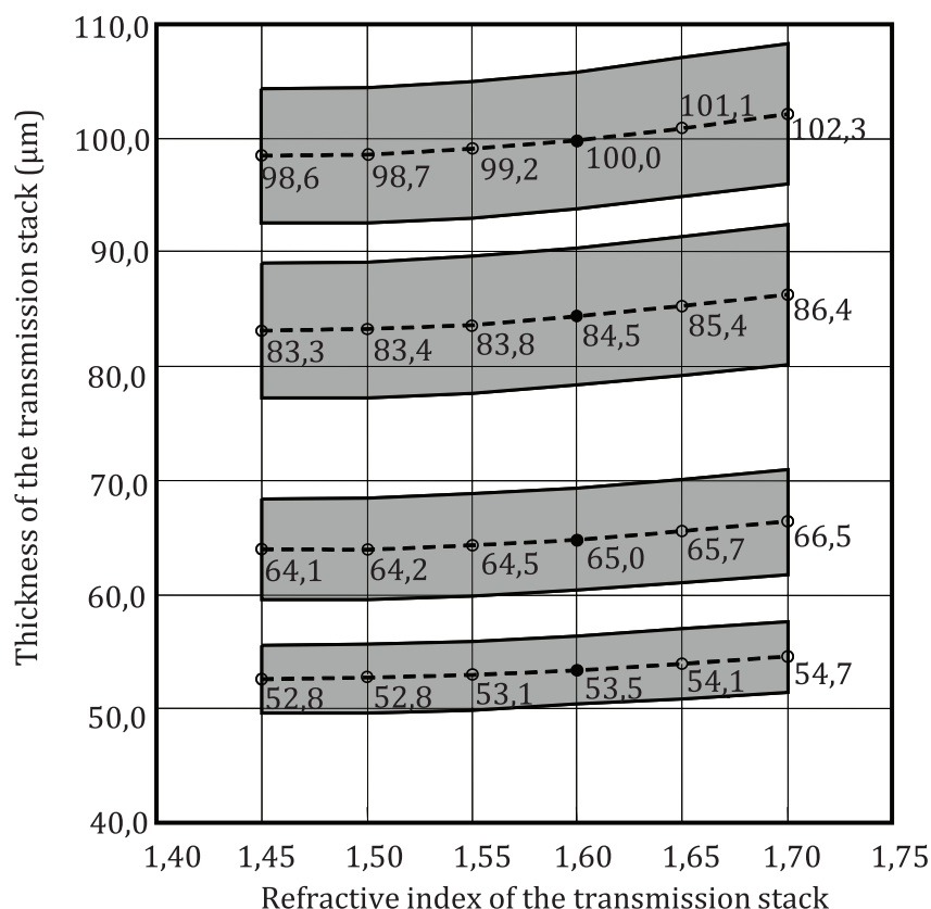
Figure 19 — Thickness of the transmission stacks as a function of the refractive index
