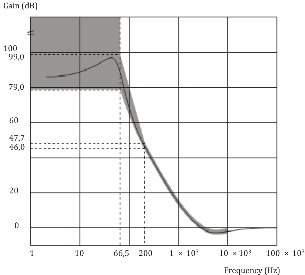
Figure 10 — Servo characteristic for radial tracking at 2x measurement velocity
