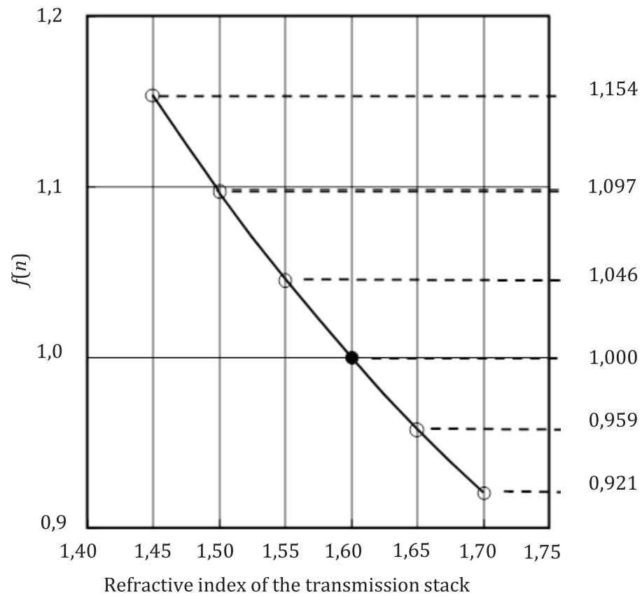
Figure 18 — Ratio of effective thickness with refractive index 1,60 and that with arbitrary refractive index n
