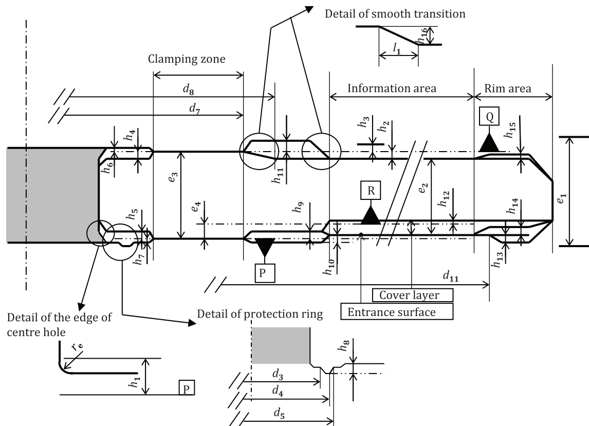
Figure 12 — Details of disk dimensions for type TL disk and type QL disk
