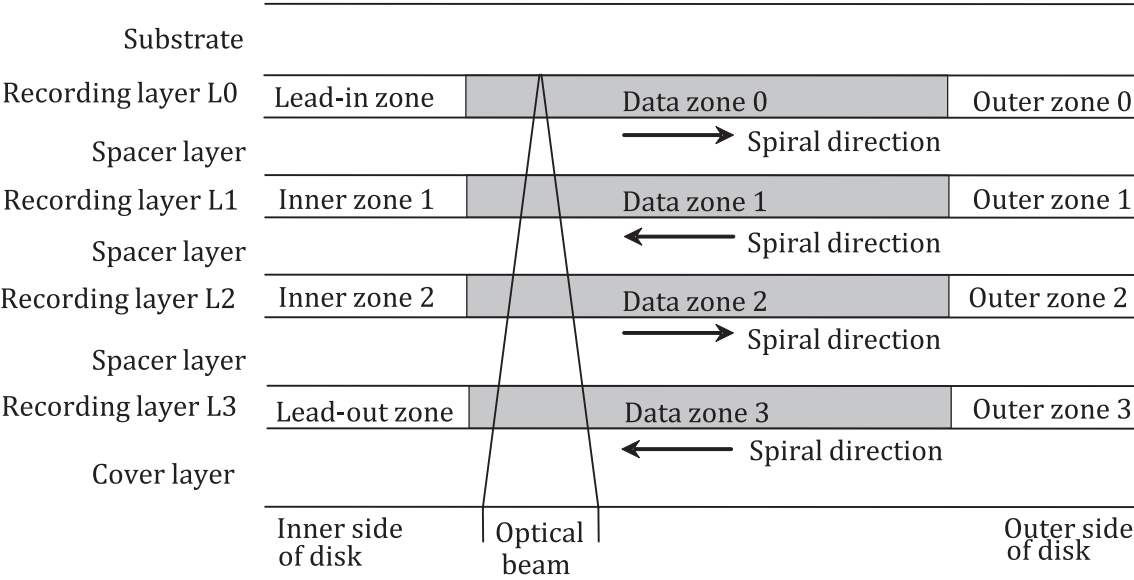
Figure 16 — Use of information area on QL disk
