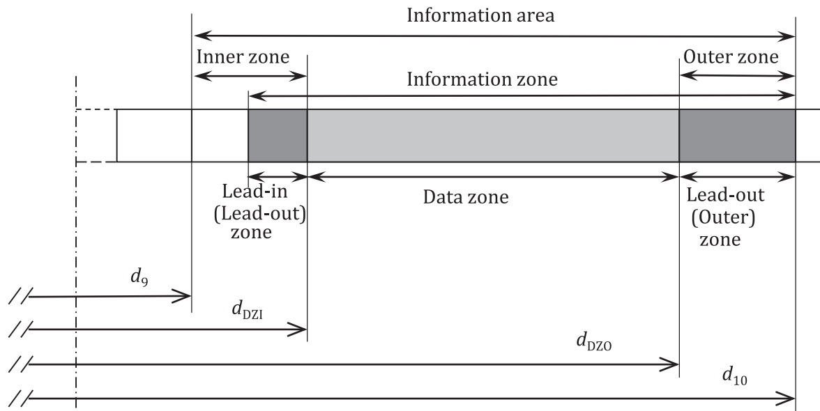
Figure 14 — Division of information area
