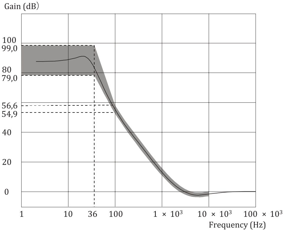
Figure 9 — Servo characteristic for radial tracking at 1x measurement velocity
