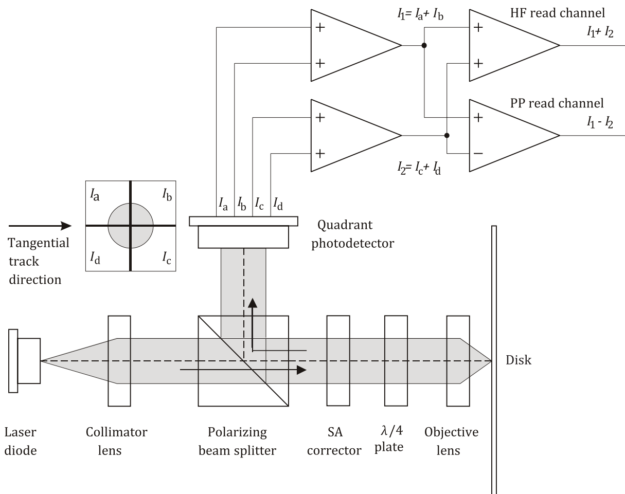
Figure 5 — Optical system of reference drive
