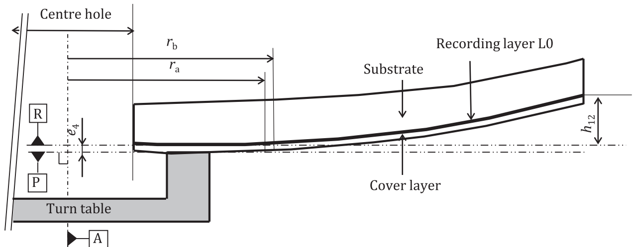
Figure 13 — Details of disk reference planes P and R and recording layer L0
