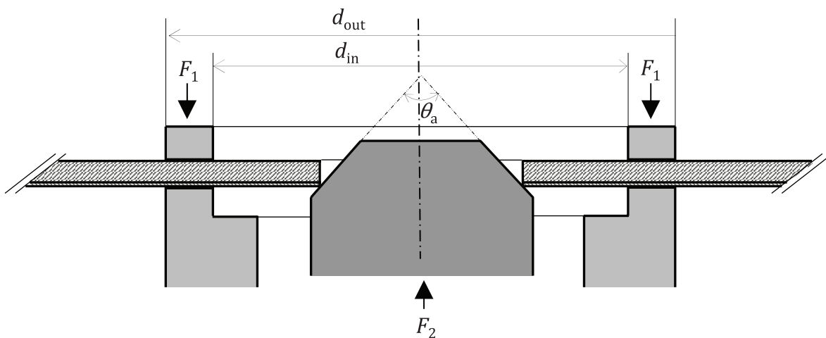
Figure 6 — Clamping conditions for measurement
