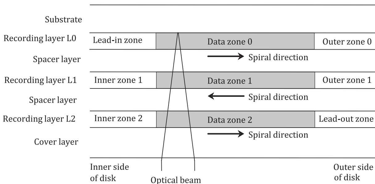
Figure 15 — Use of information area on TL disk
