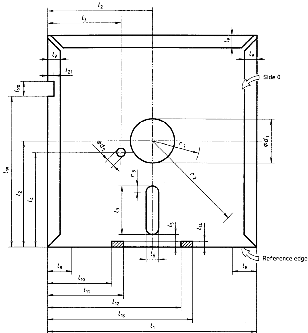
Figure 3 — Jacket dimensions
