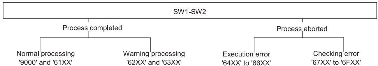
Figure 2 — Structural scheme of values of SW1-SW2
