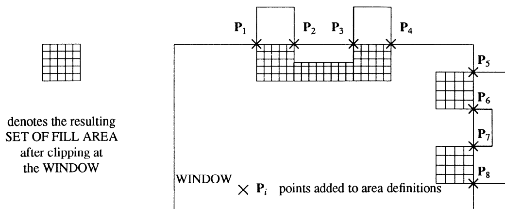
Figure 9 - Example of SET OF FILL AREA scissoring
