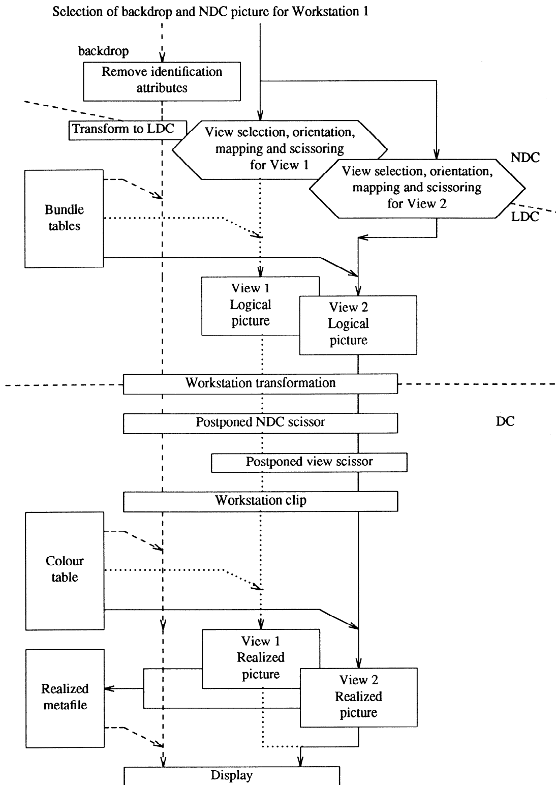
Figure 4 - GKS logical and realized pictures
