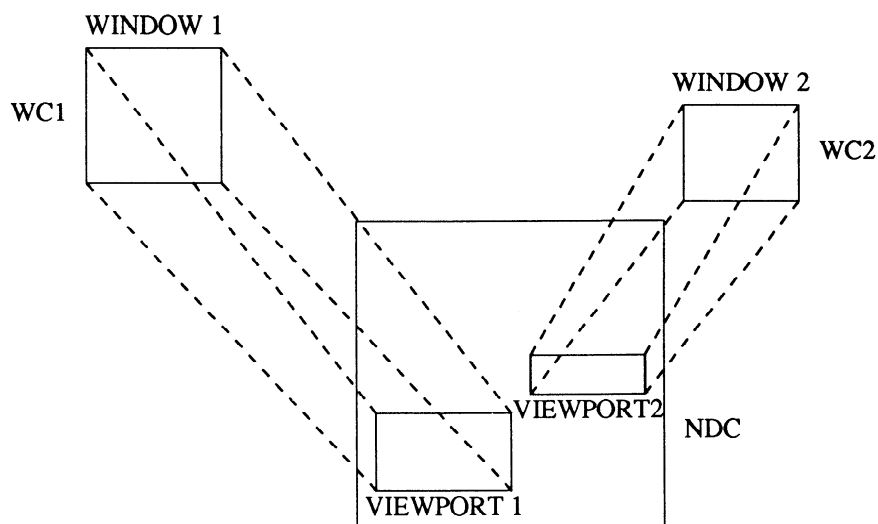
Figure 5 - Normalization transformations
