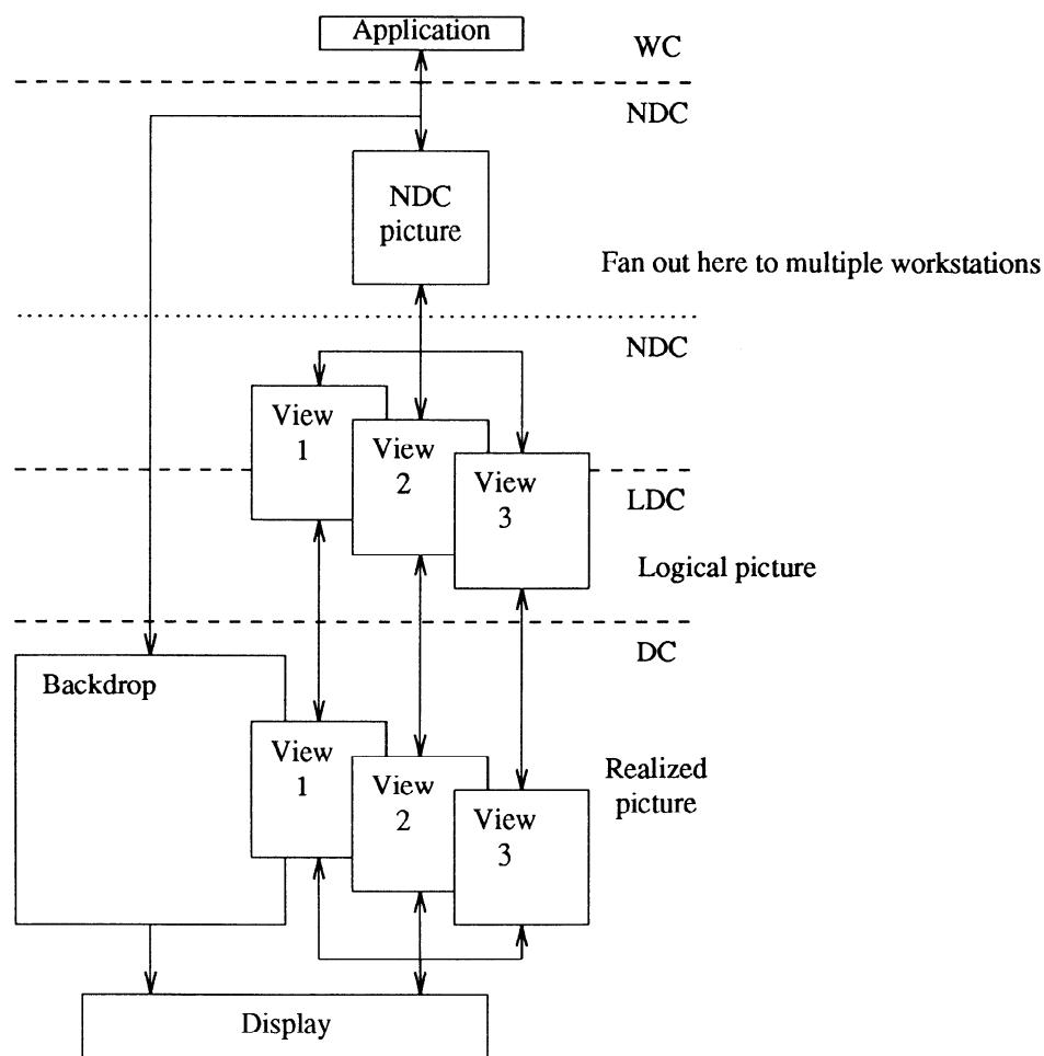
Figure 2 - GKS overview
