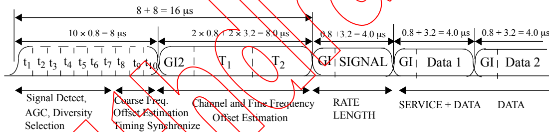
Figure 110—OFDM training structure
