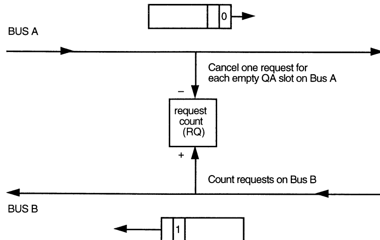
Figure 2-4a)—Node not queued to send (Bus A)
