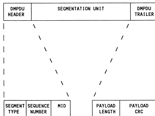
Figure 2-9—Format of a DMPDU
