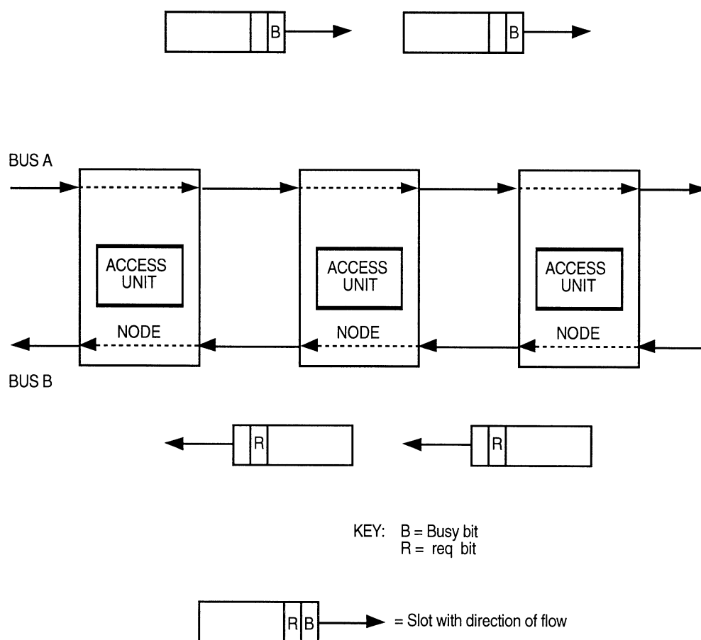
Figure 2-3—Queue formation on Bus A
