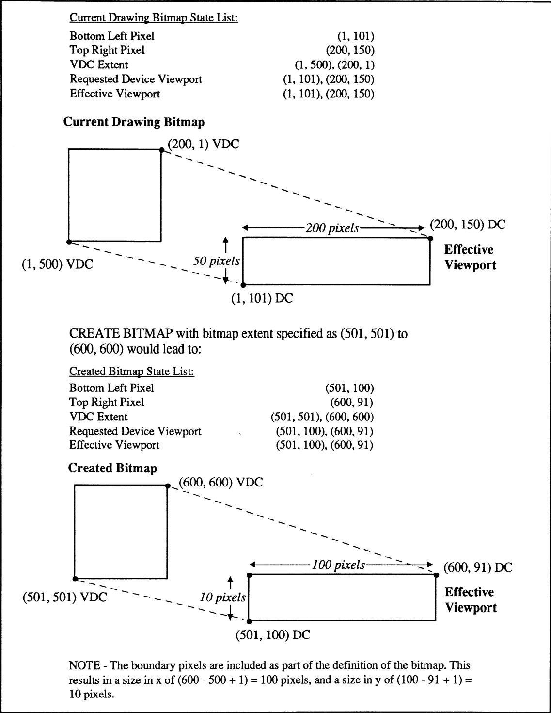
Figure 5 – Creating bitmaps
