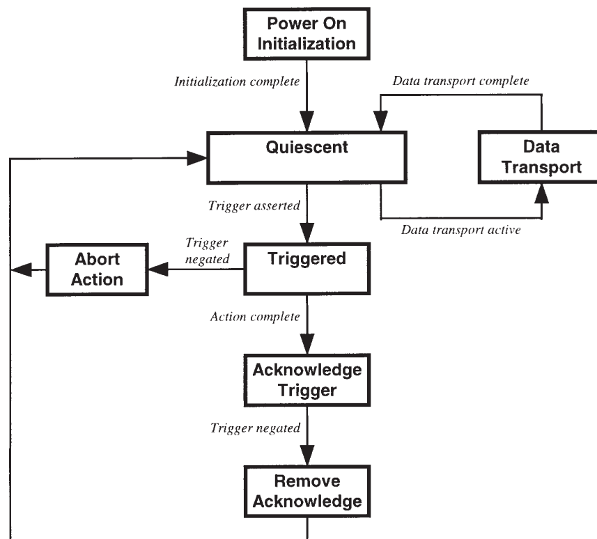
Figure 3—General response of STIM to a trigger
