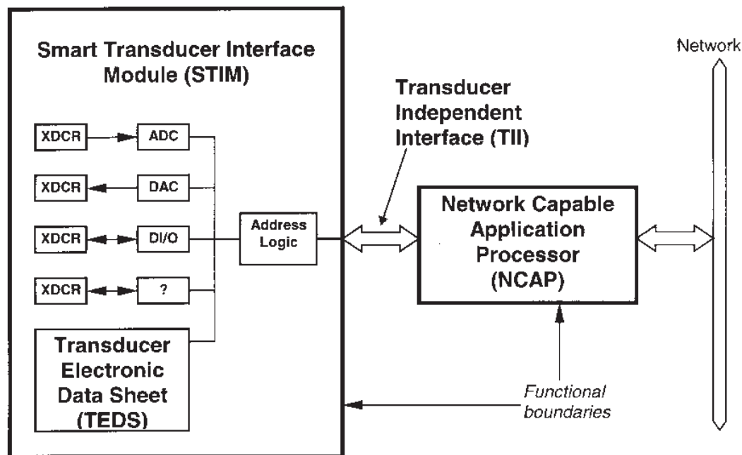
Figure 1—Context for the transducer interface specification
