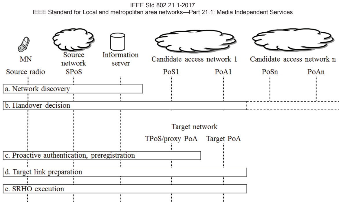
Figure 3—Single-radio handover procedures
