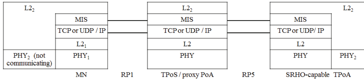
Figure 5—Transport of the L2 frame of the target interface via a MIS using the logical connection at the TPoS to the SRHO-capable TPoA
