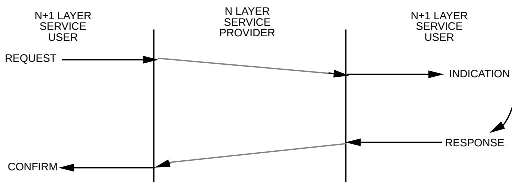
f) Cycle of interactions between peer entities
