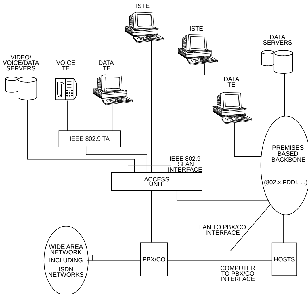
Figure 5-2—IEEE 802.9 ISLAN interface configuration
