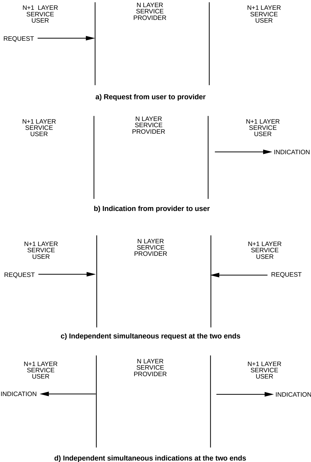
Figure 1-4—Timing relationship between service primitives
