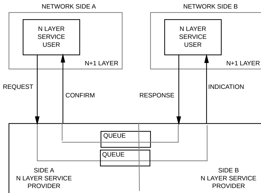
Figure 1-3—End-to-end relationship of service primitives
