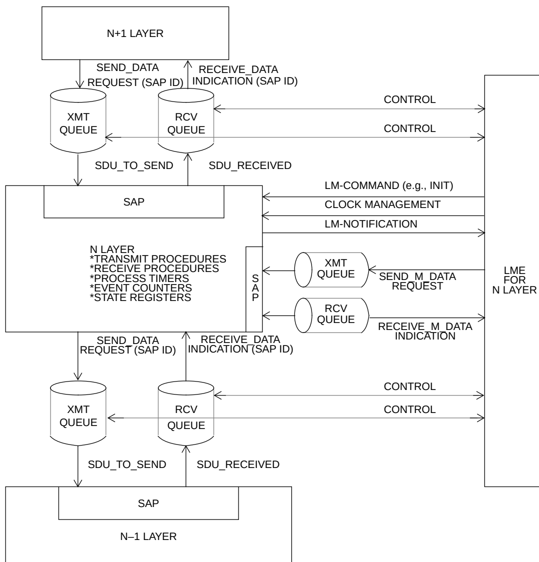
Figure 1-5—Service queues between adjacent layers
