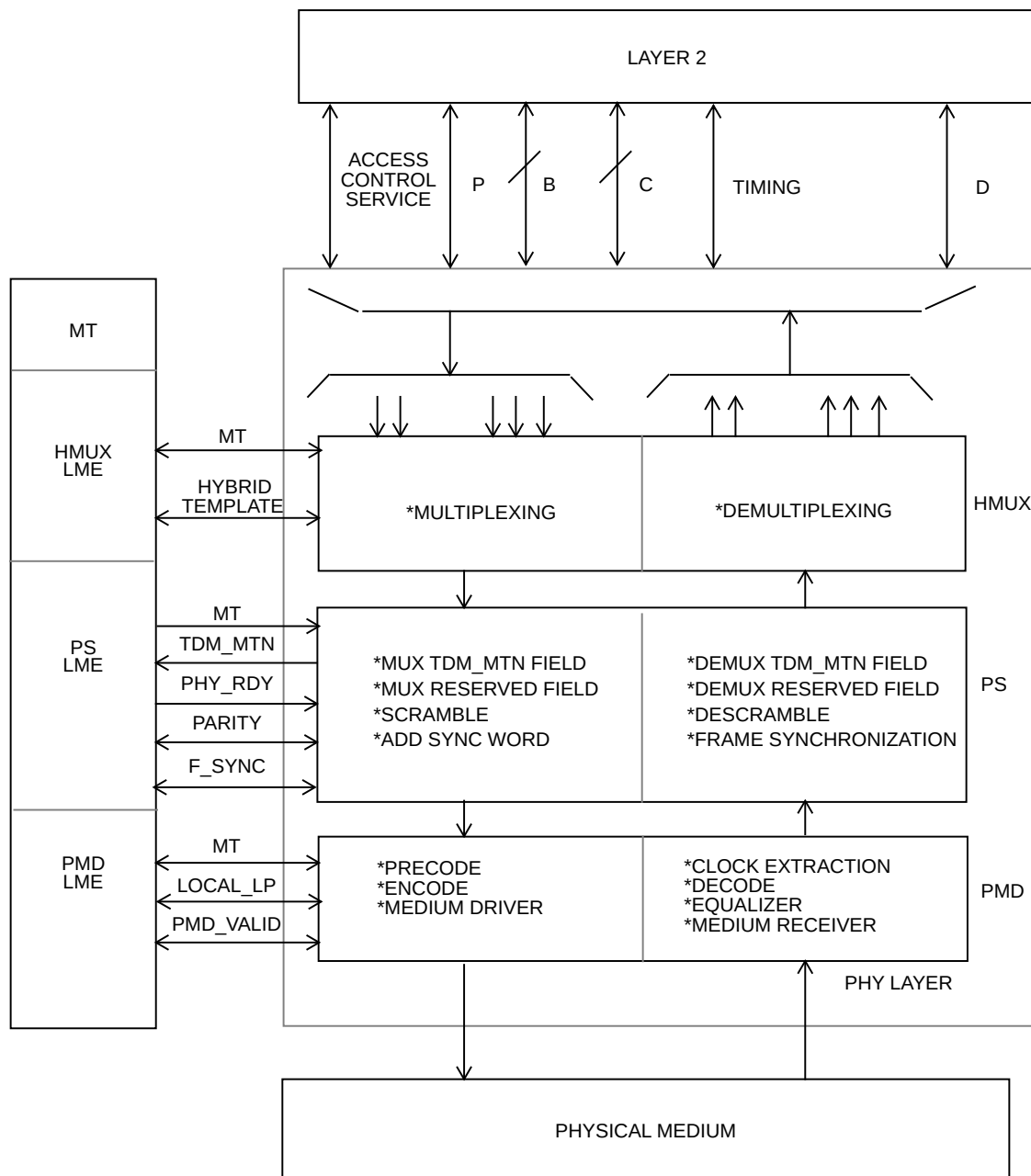
Figure 5-5—IEEE 802.9 ISLAN interface configuration
