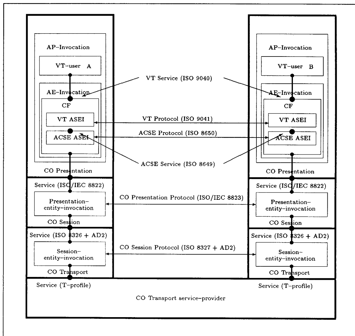
Figure 1 — Interactive VT communication between two end systems
