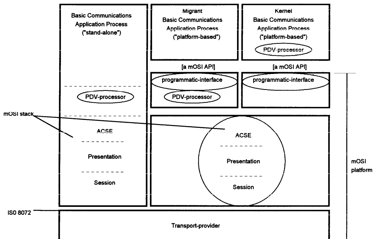
Figure 1 -- mOSI model
