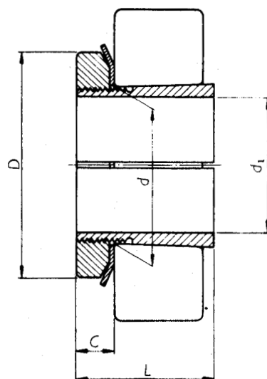
Adapter sleeve
