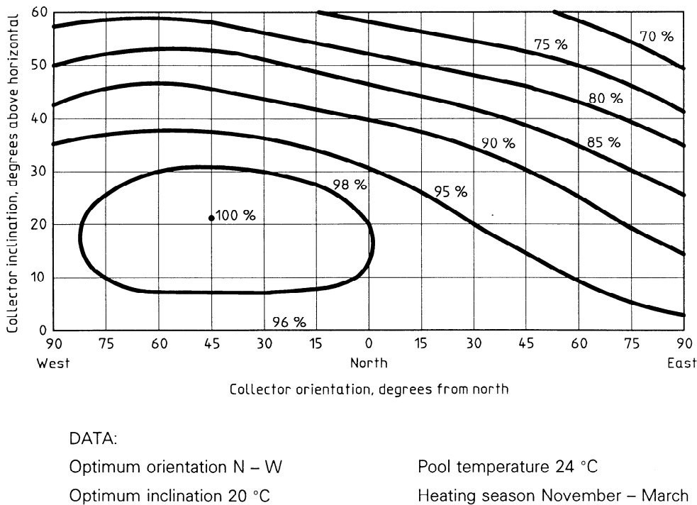
Figure 3 — Relative collector output as a function of orientation and inclination (for southern hemisphere)
