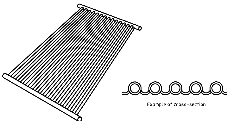
Figure 1 — Example of a plastic/elastomeric panel collector
