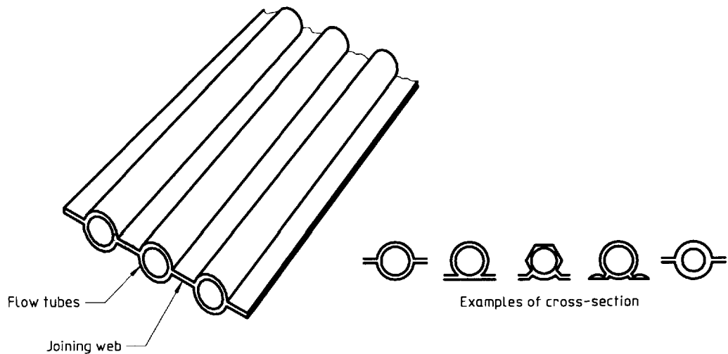
Figure 2 — Plastic strip collector
