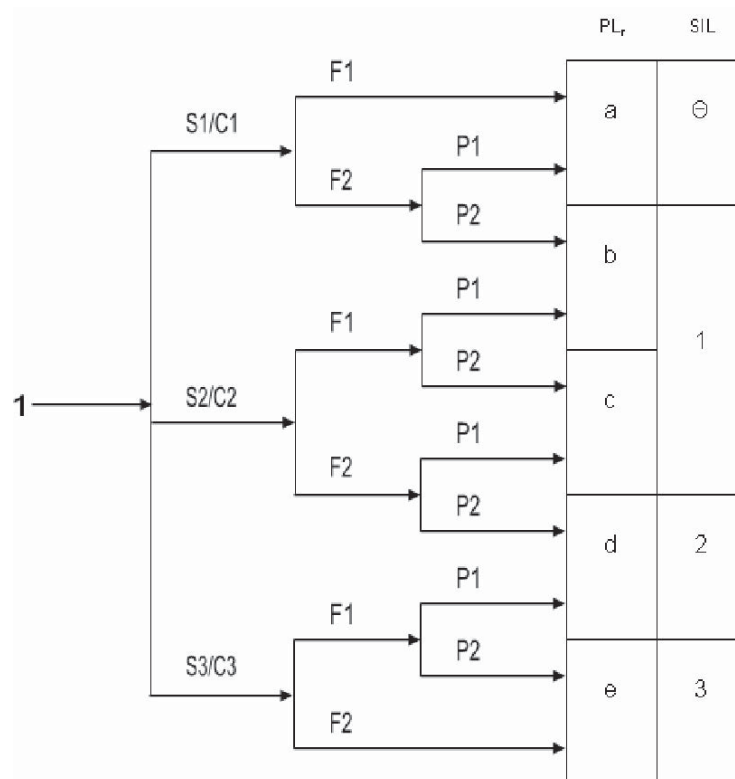
Figure 1 — Risk graph
