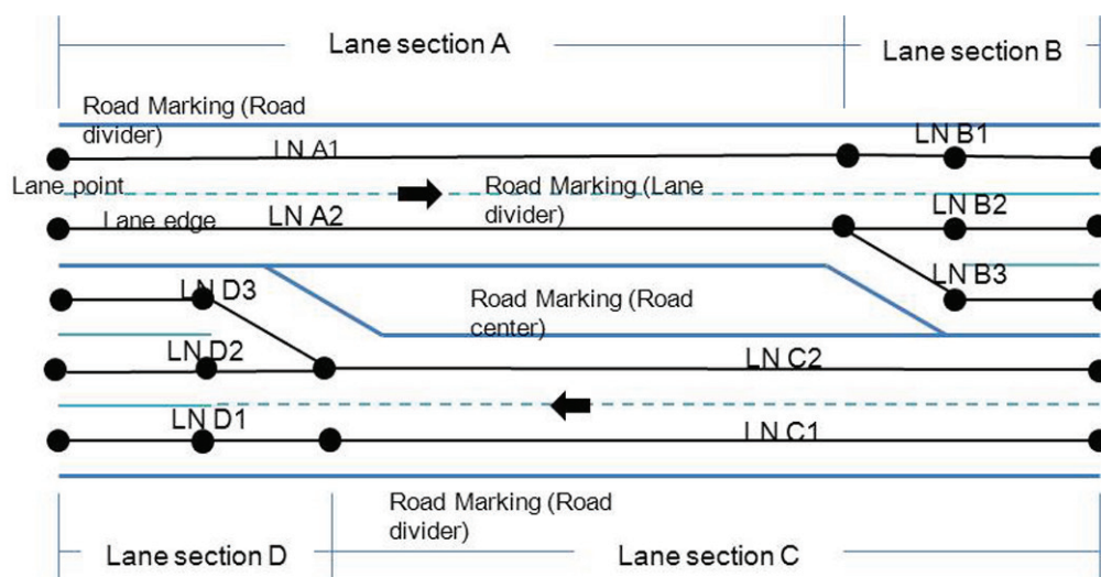
Figure 5 — Lane structure
