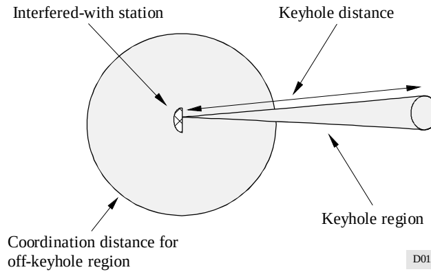
FIGURE 1 Basic concept for keyhole coordination distance
