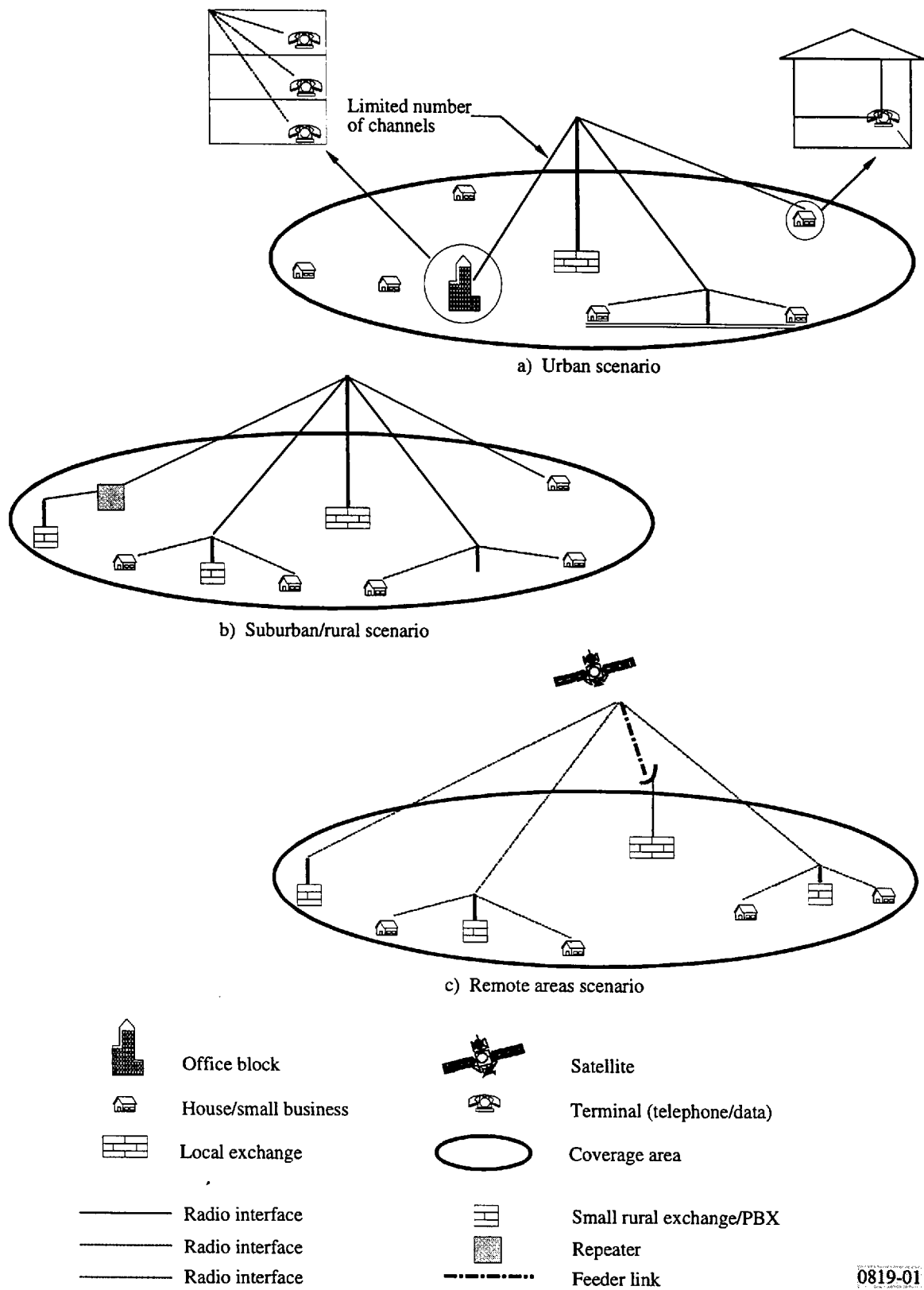
FIGURE 1 Some possible uses of IMT-2000 radio interfaces for network wireless access in the fixed service
