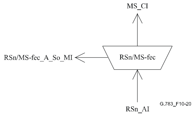
Figure 10-20/G.783 – RSn/MS-fec_A_Sk symbol
