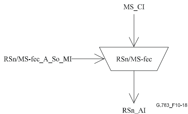
Figure 10-18/G.783 – RSn/MS-fec_A_So symbol
