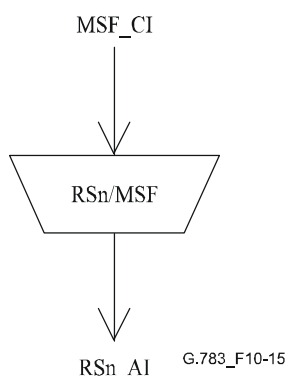
Figure 10-15/G.783 – RSn/MSF_A_So symbol
