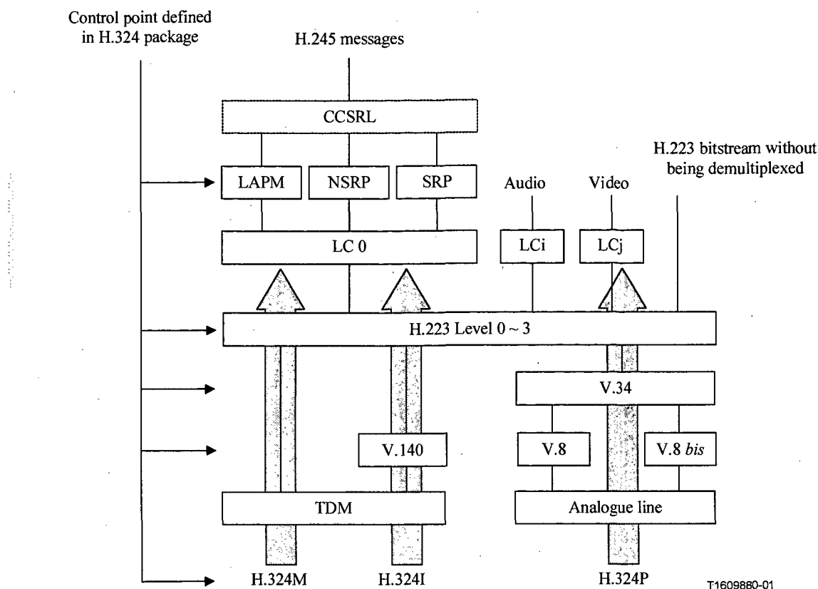
Figure 1/H.248.12 – Control point defined in H.324 package
