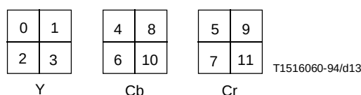
Figure 6-12 – 4:4:4 Macroblock structure
