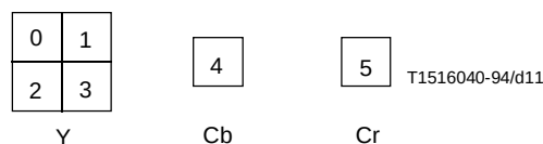
Figure 6-10 – 4:2:0 Macroblock structure
