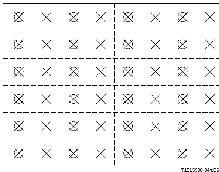
Figure 6-5 – The position of luminance and chrominance samples – 4:2:2 data
