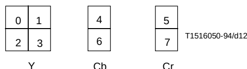
Figure 6-11 – 4:2:2 Macroblock structure
