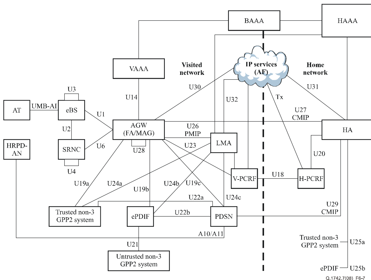
Figure 6-7 – Converged Access Network Reference Model – Roaming
