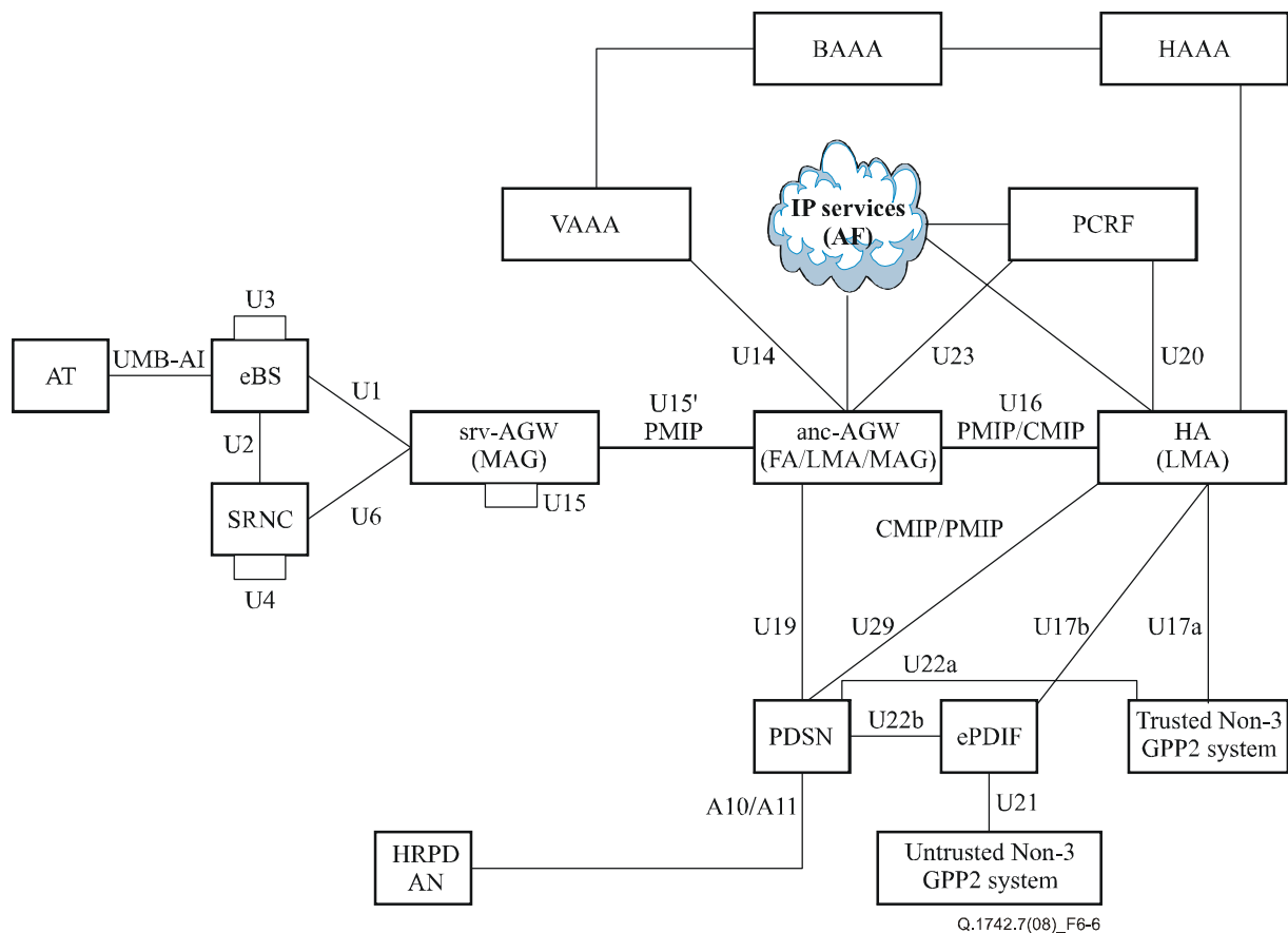
Figure 6-6 – Converged Access Network Reference Model, non-Roaming
