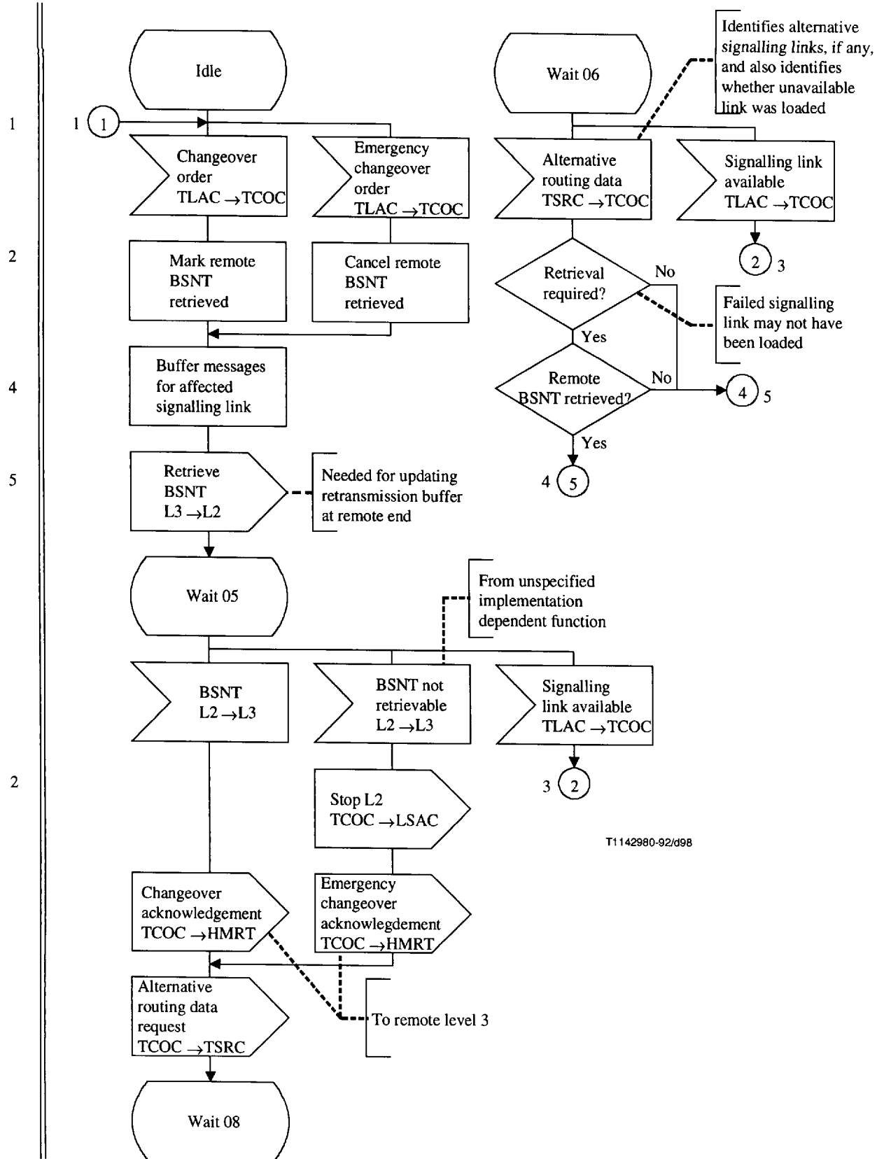
Figure 30/Q.704 (sheet 6 de 6) – Signalling traffic management; changeover control (TCOC)
