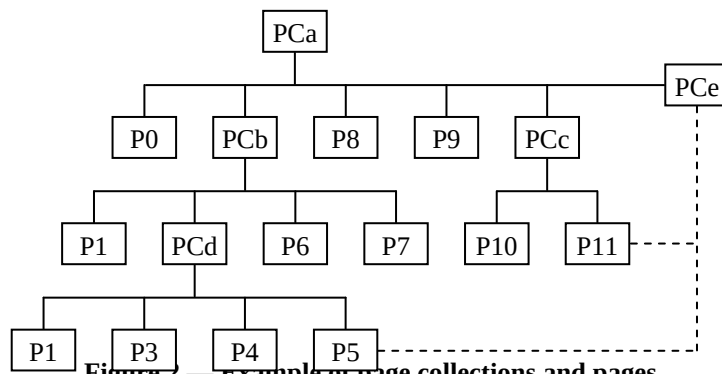
Figure 2 — Example of page collections and pages
