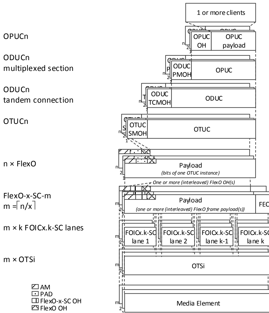
Figure 7-1 – FlexO-x-SC-m interface group principal information containment relationship
