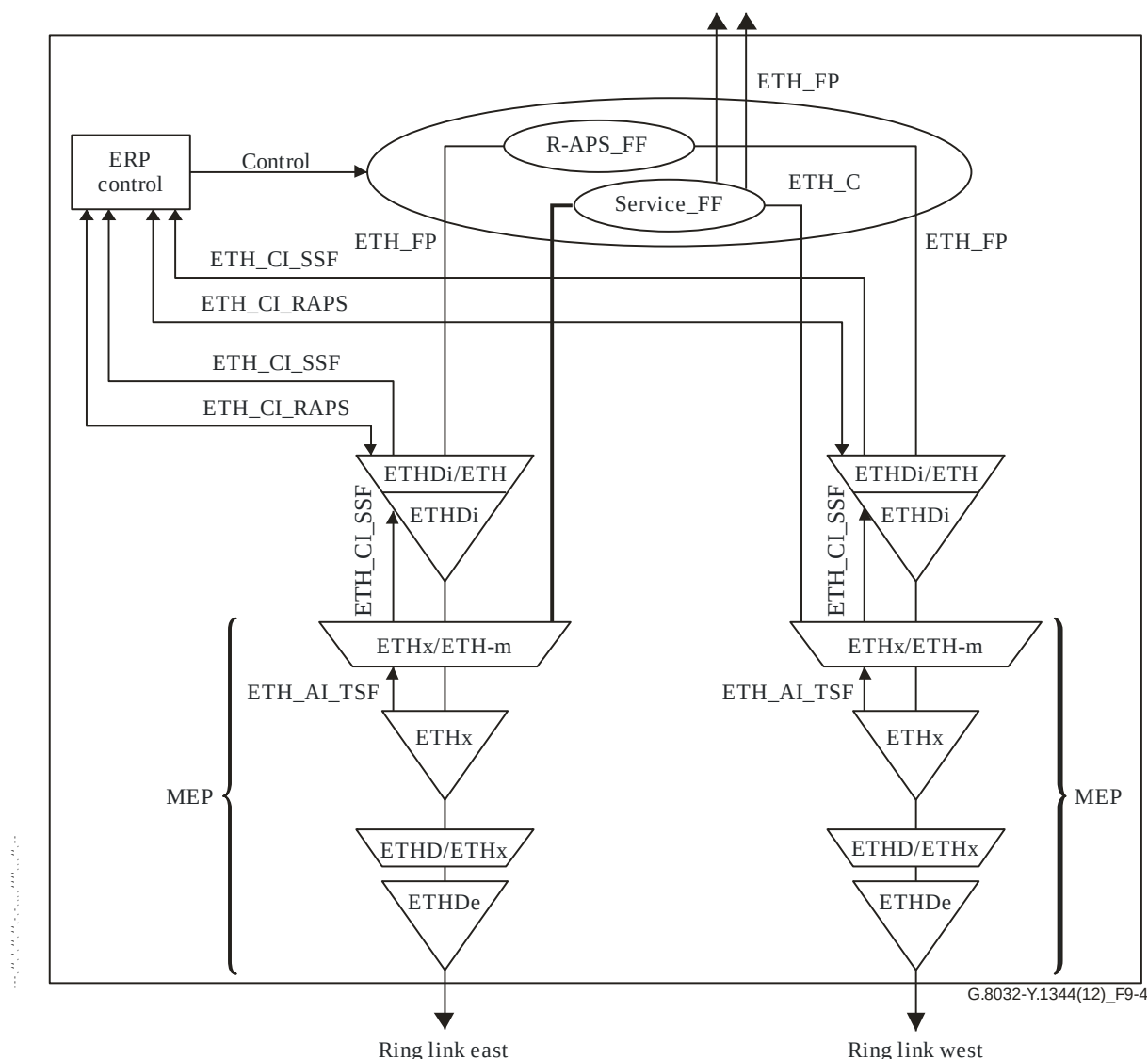
Figure 9-4 – MEPs and R-APS insertion function in Ethernet ring node (normal Ethernet ring node)
