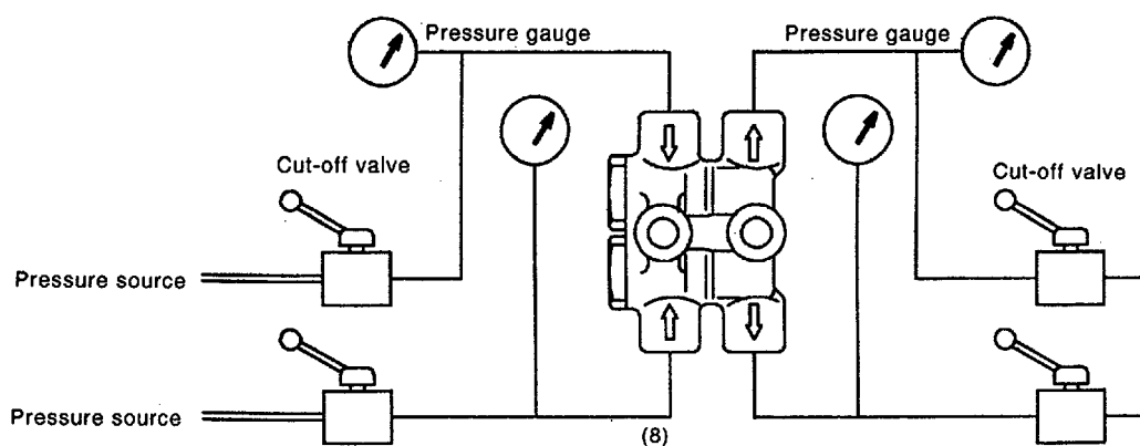
Fig. 5 Pressure device for airtightness
