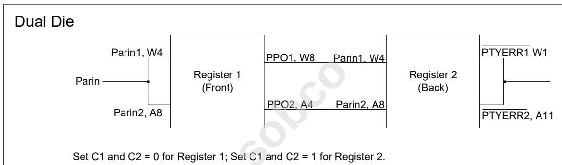
Figure 1 — Parity Implementation and Device Wiring for SSTUA32S869 and SSTUA32D869
