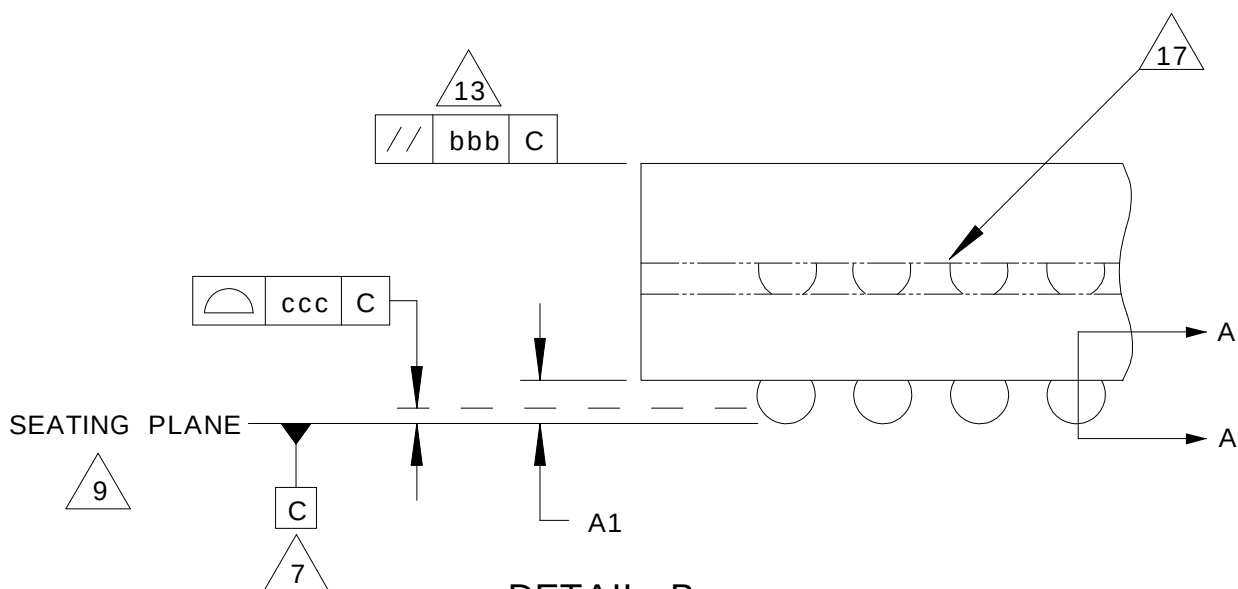
DETAIL B (ROTATED 90° CW)
