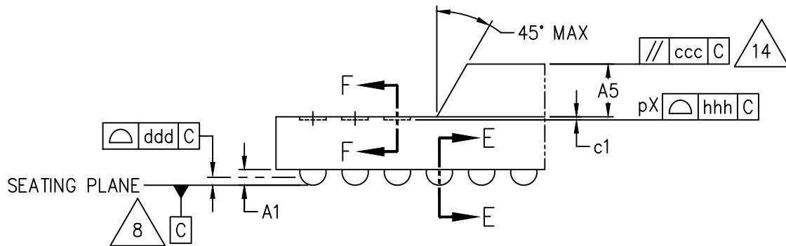
DETAIL B WITH FLANGED TYPE MOLD CAP (ROTATED 90° CW)
