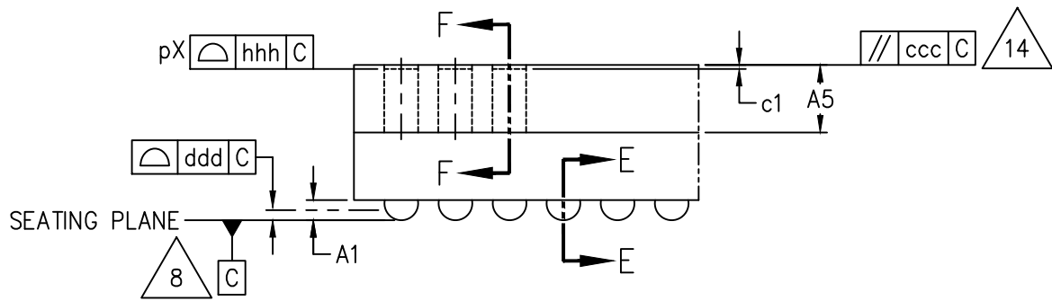
DETAIL B WITH THROUGH VIA MOLD CAP (ROTATED 90° CW)
