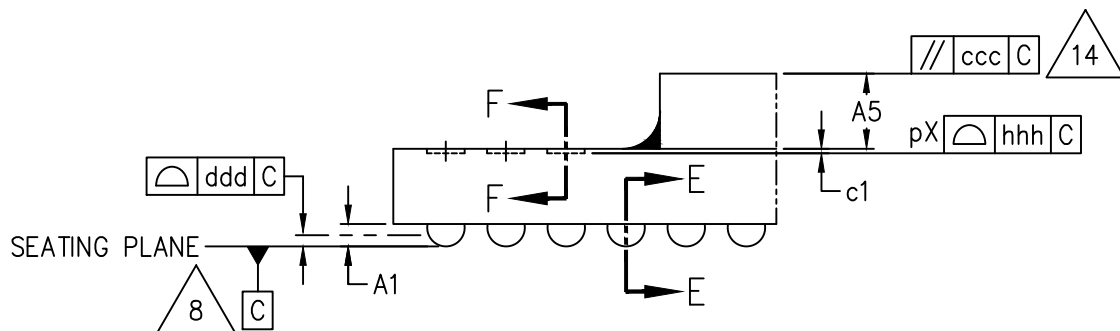
DETAIL B WITH BARE DIE (ROTATED 90° CW)
