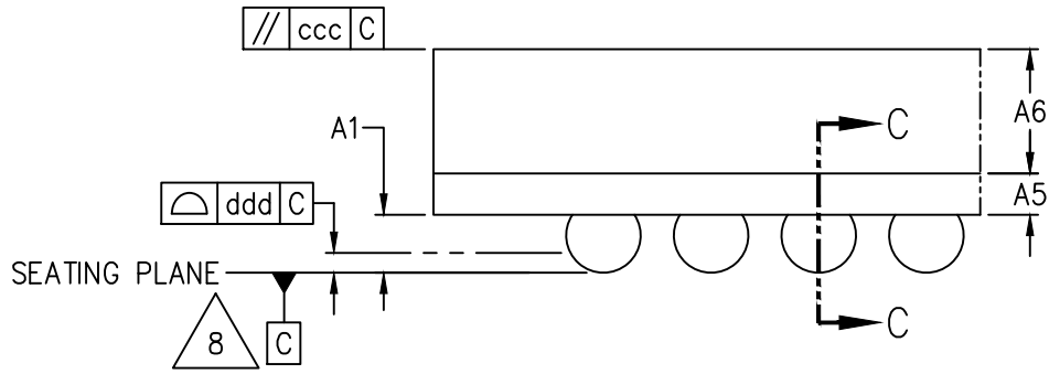
DETAIL A (ROTATED 90° CW)
