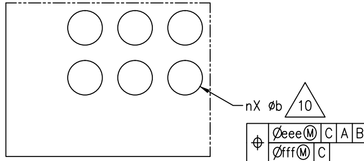
DETAIL B
