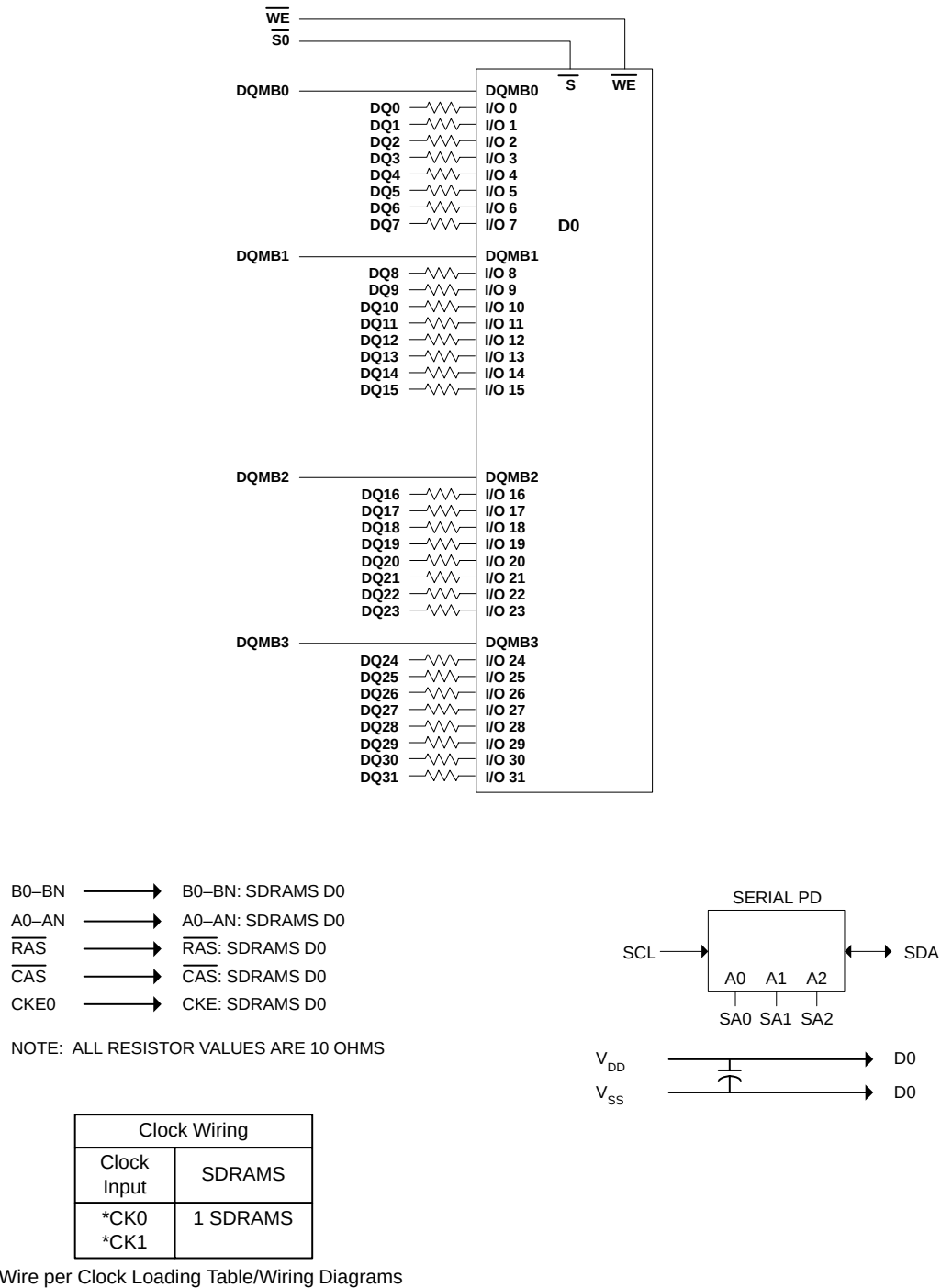
Figure 4.4.8-I 100 Pin X32 SDRAM DIMM, 1 Bank with X32 SDRAMs
