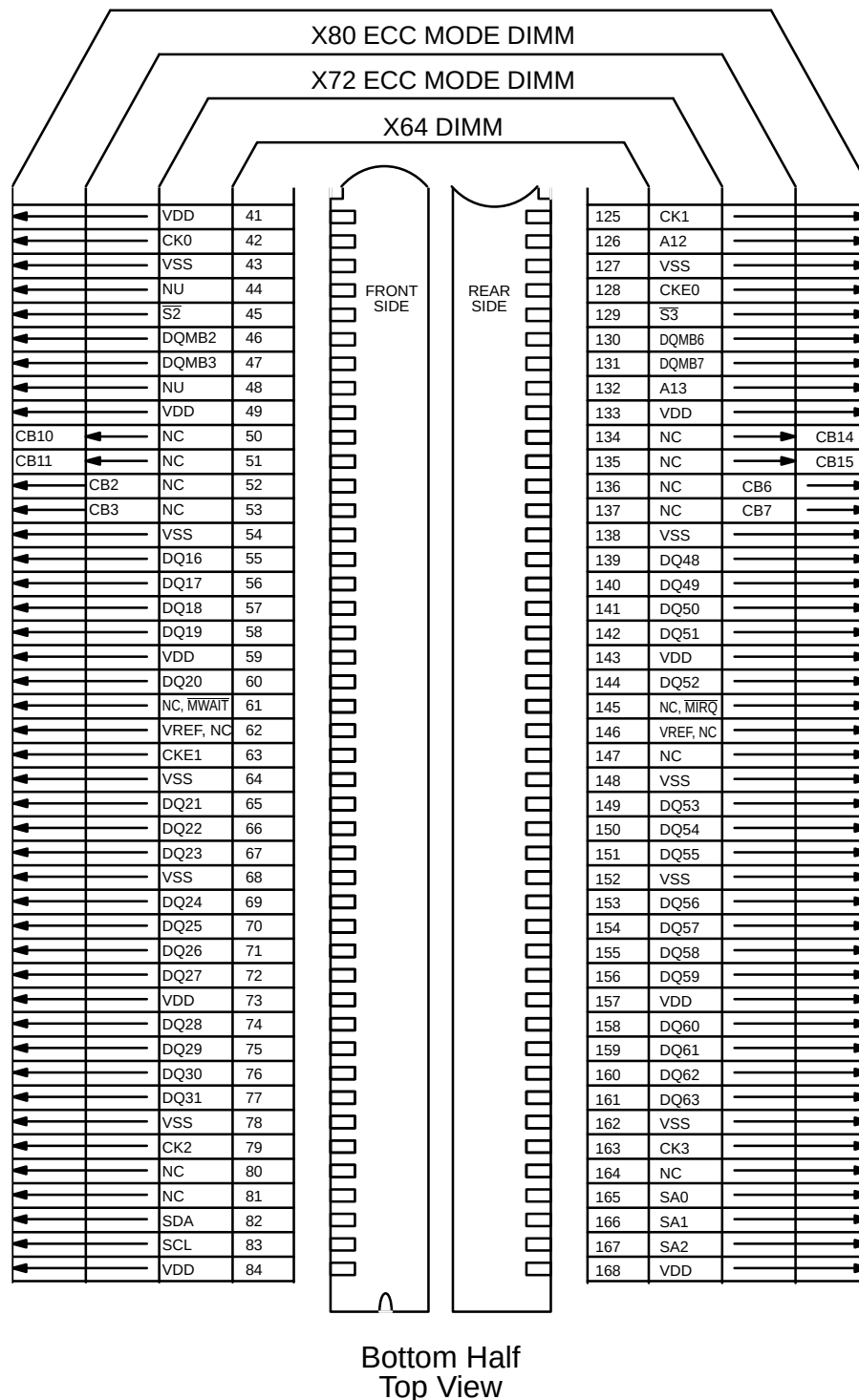
FIGURE 4.5.4-B 168 PIN, 64, 72, or 80 BIT SDRAM DIMM PINOUT, BOTTOM HALF
