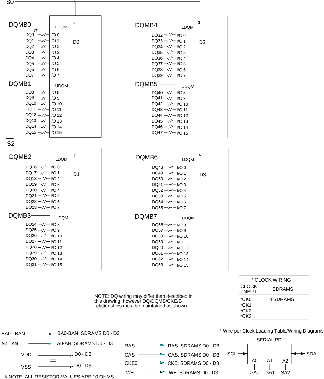
Figure 4.5.4-K X64 SDRAM DIMM, 1 Bank with X16 SDRAMs
