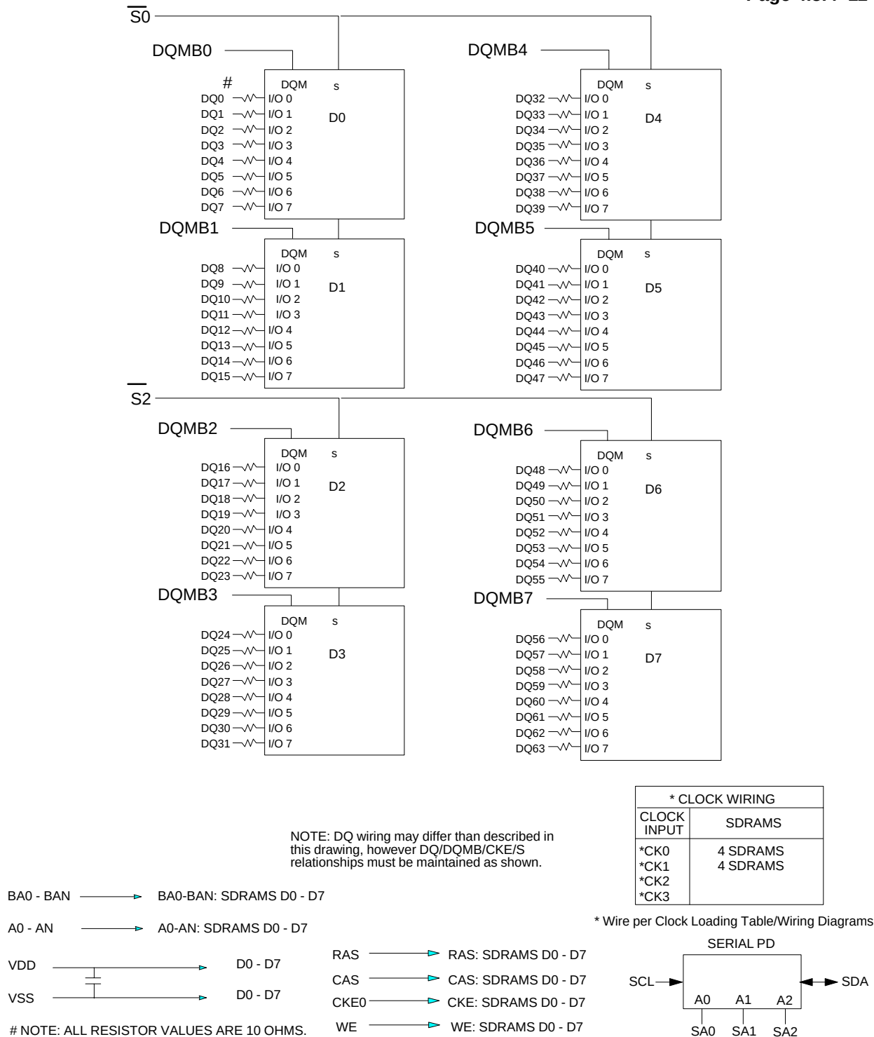
Figure 4.5.4-J X64 SDRAM DIMM, 1 Bank with X8 SDRAMs
