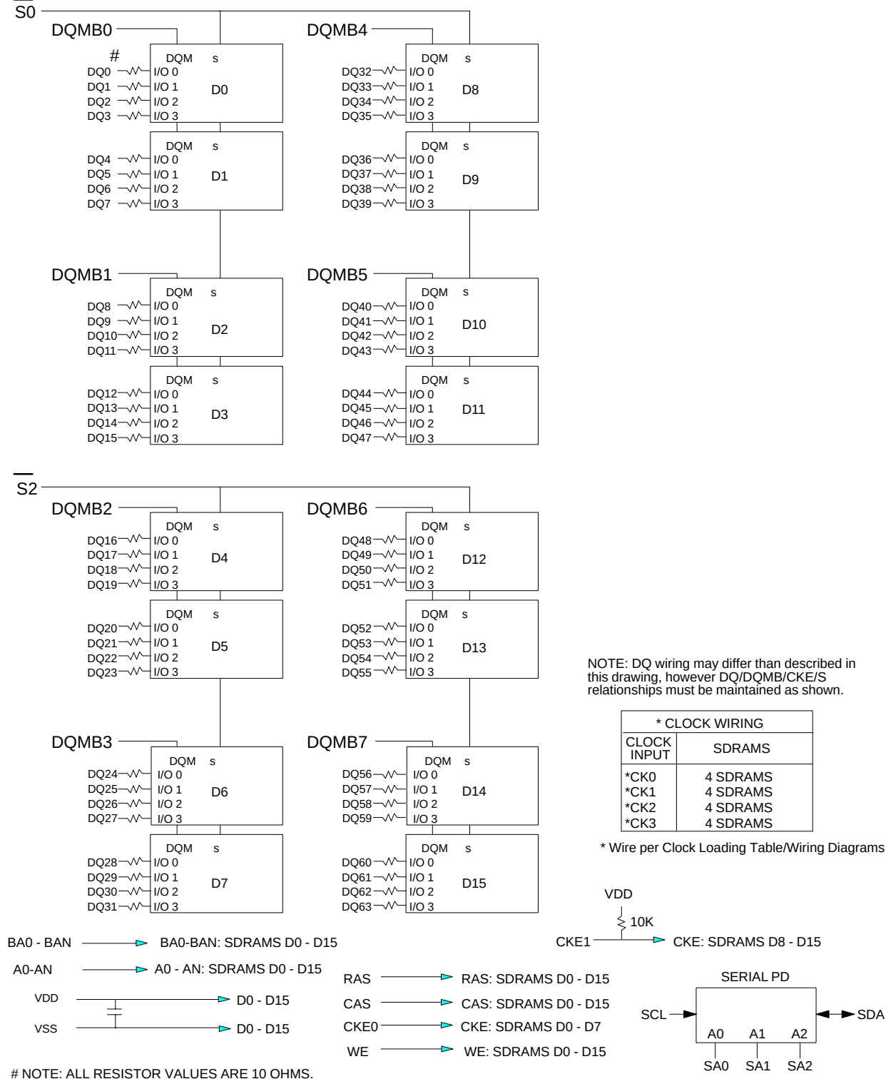
Figure 4.5.4-I X64 SDRAM DIMM, 1 Bank with X4 SDRAMs
