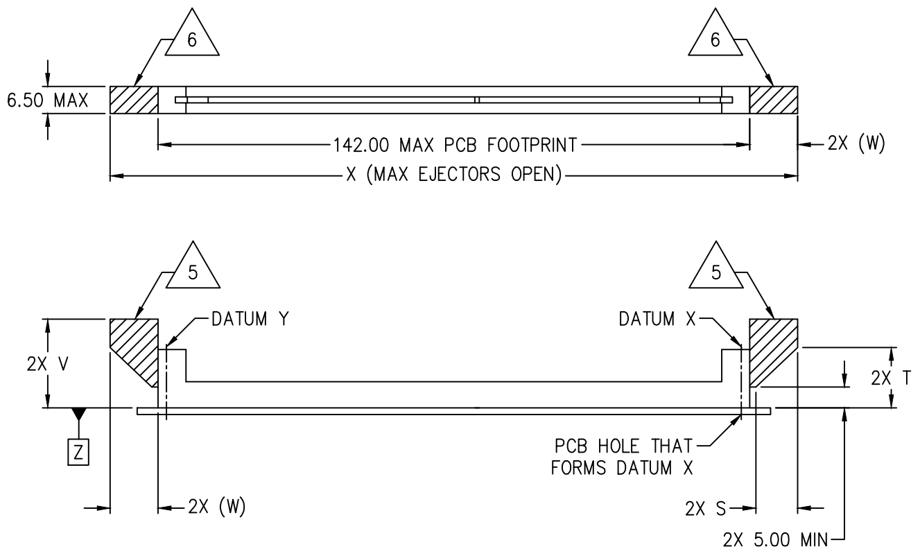
SIDE VIEW (PCB AND SOCKET)
