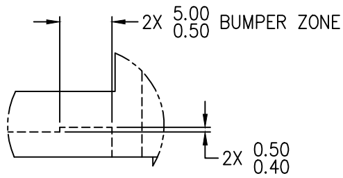
DETAIL F
