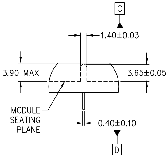
DETAIL D
