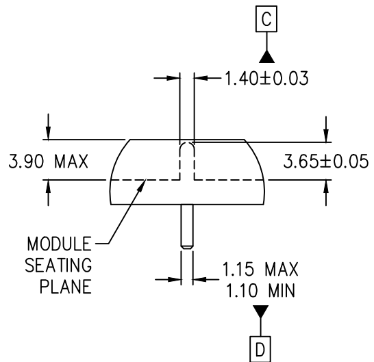
DETAIL E
