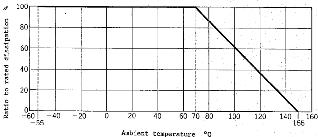
Fig. 1. Derating Curve
